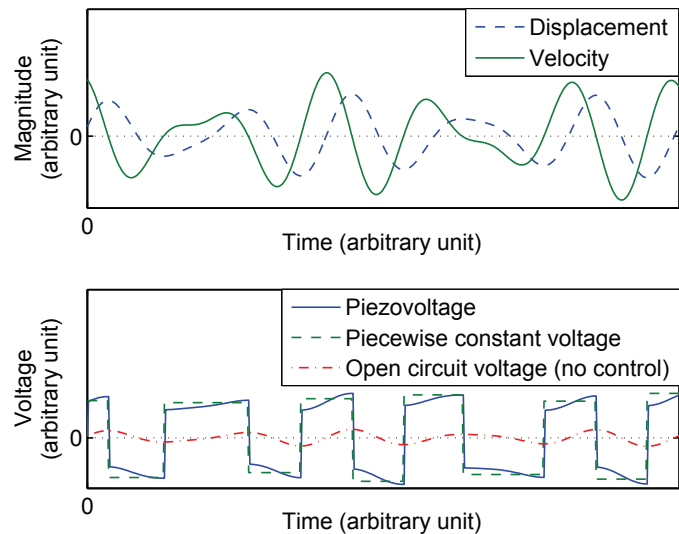
Fig. 2. Waveforms using nonlinear treatment
