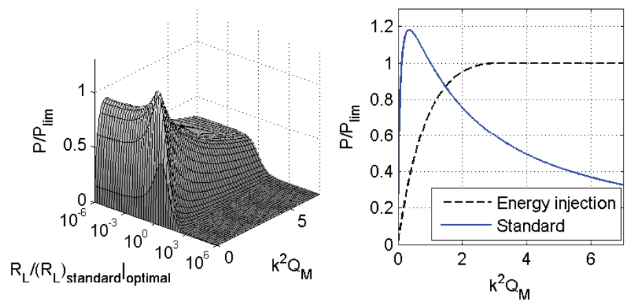
Fig. 15. Normalized harvested power and maximal normalized harvested power of energy injection technique under constant force magnitude and comparison with standard interface ( \gamma = 0.8, \gamma_C = 0.9 )
