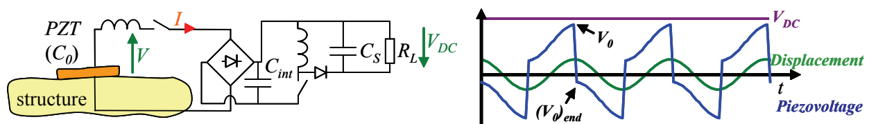
Fig. 10. DSSH technique and waveforms
