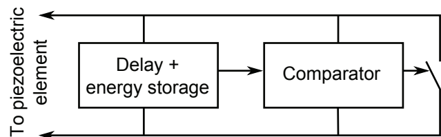
Fig. 16. Principles of the self-powered switch
