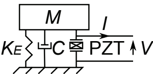
Fig. 1. Single Degree Of Freedom (SDOF) model of an electromechanical structure
