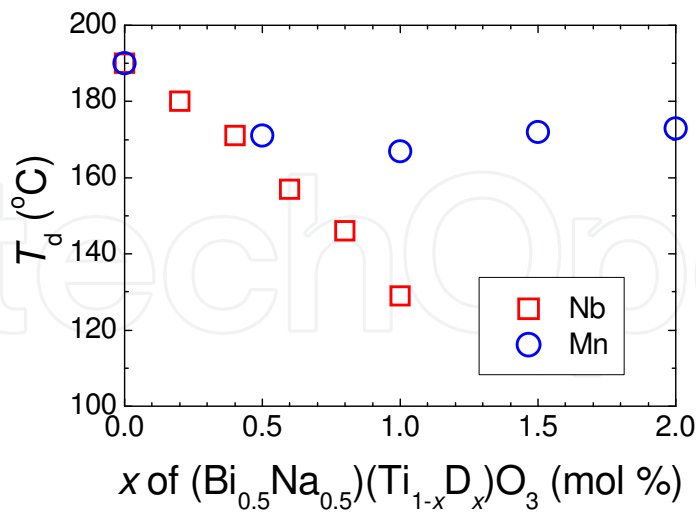
Fig. 7. Depolarization temperature ( T_d ) of (\text{Bi}_{0.5}\text{Na}_{0.5})(\text{Ti}_{1-x}\text{D}_x)\text{O}_3 ceramics ( \text{D} = \text{Nb}, \text{Mn} )
