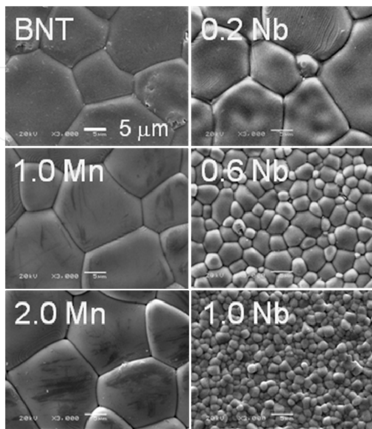
Fig. 2. SEM secondary electron images of the surfaces of (\text{Bi}_{0.5}\text{Na}_{0.5})(\text{Ti}_{1-x}\text{D}_x)\text{O}_3 pellets ( \text{D} = \text{Nb, Mn} ) sintered at 1150^\circ\text{C} for 2 h in air
