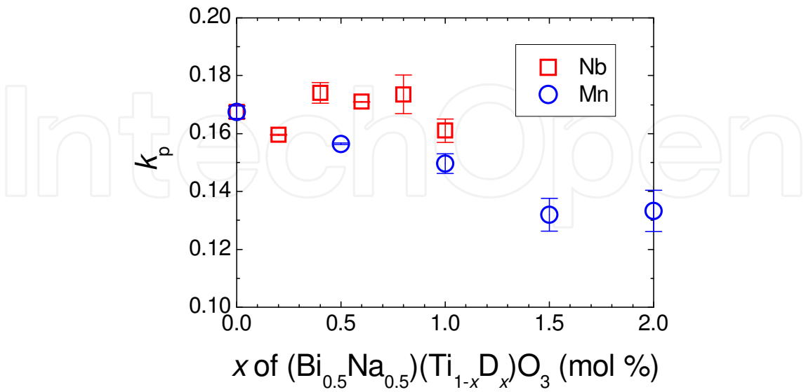
Fig. 4. Electromechanical coupling factor ( k_p ) of (Bi 0.5 Na 0.5 )(Ti 1-x D x )O 3 ceramics (D = Nb, Mn)
