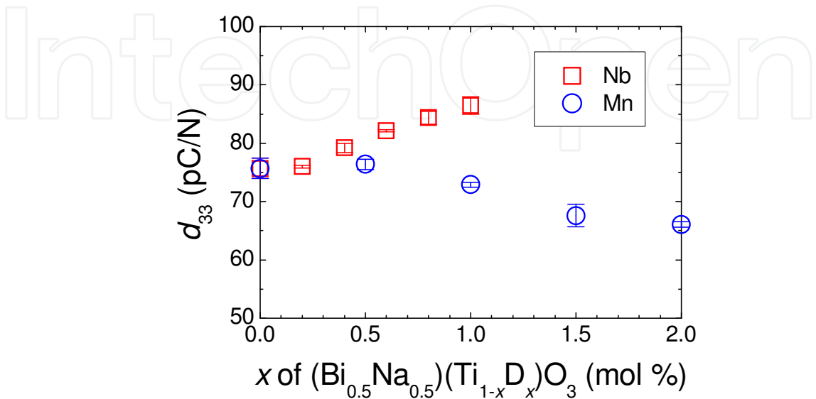
Fig. 3. Piezoelectric coefficient ( d_{33} ) of (Bi 0.5 Na 0.5 )(Ti 1-x D x )O 3 ceramics (D = Nb, Mn)
