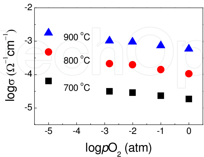
Fig. 8. Electrical conductivity ( \sigma ) of BNT ceramics as a function of oxygen partial pressure ( p\text{O}_2 ) at 700, 800, and 900 ^\circ\text{C}
