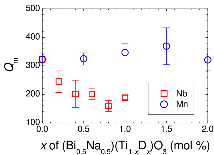
Fig. 5. Mechanical quality factor ( Q_m ) of (\text{Bi}_{0.5}\text{Na}_{0.5})(\text{Ti}_{1-x}\text{D}_x)\text{O}_3 ceramics ( \text{D} = \text{Nb}, \text{Mn} )
