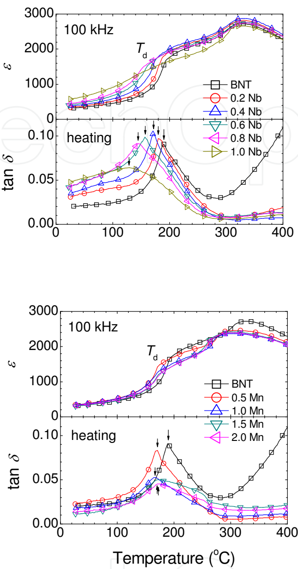
Fig. 6. Dielectric constant ( \epsilon ) and loss tangent ( \tan \delta ) of (\text{Bi}_{0.5}\text{Na}_{0.5})(\text{Ti}_{1-x}\text{D}_x)\text{O}_3 ceramics (D = Nb, Mn). Arrow marks indicate the depolarization temperature ( T_d )
