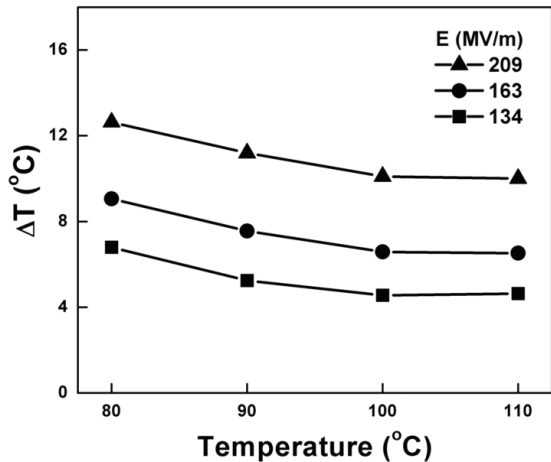
Fig. 7. Adiabatic temperature changes as a function of ambient temperature at different electric fields.
