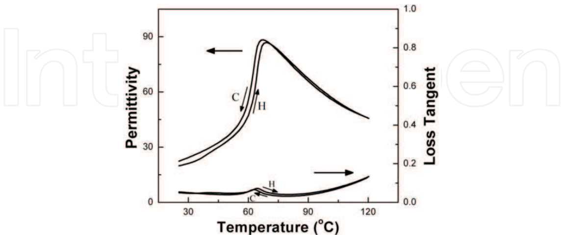
Fig. 2. Permittivity as a function of temperature for P(VDF-TrFE) 55/45 mol% copolymers.
