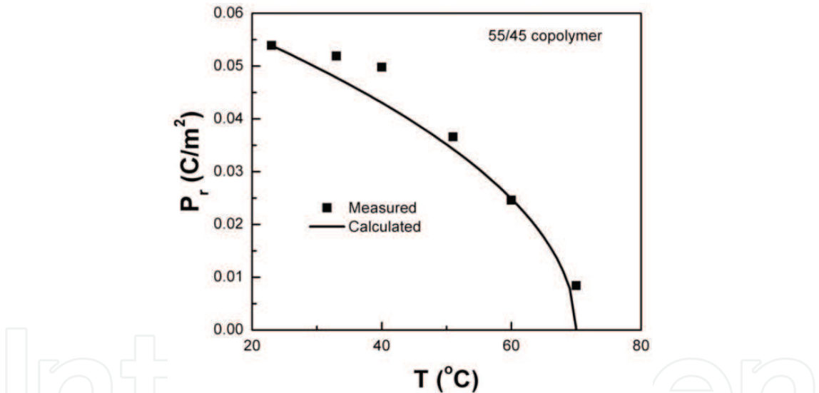
Fig. 3. Remanent polarization as a function of temperature for P(VDF-TrFE) 55/45 mol% copolymers.
