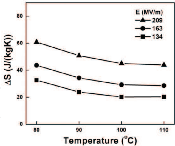
Fig. 6. Isothermal entropy changes as a function of ambient temperature at different electric fields.
