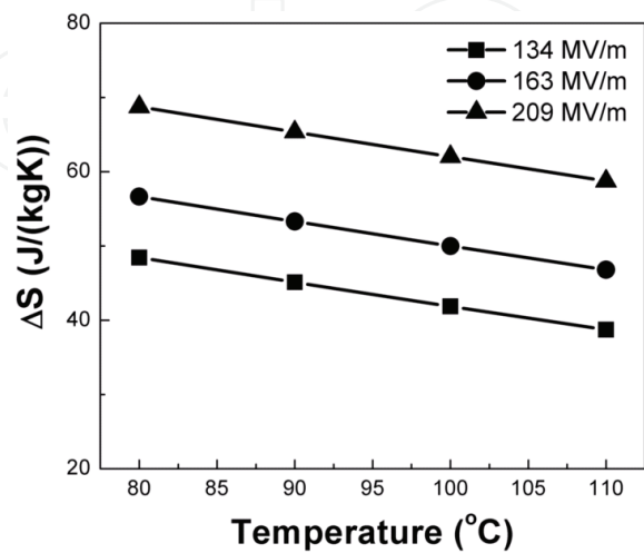
Fig. 11. ECE entropy changes versus temperature for 55/45 copolymer.
