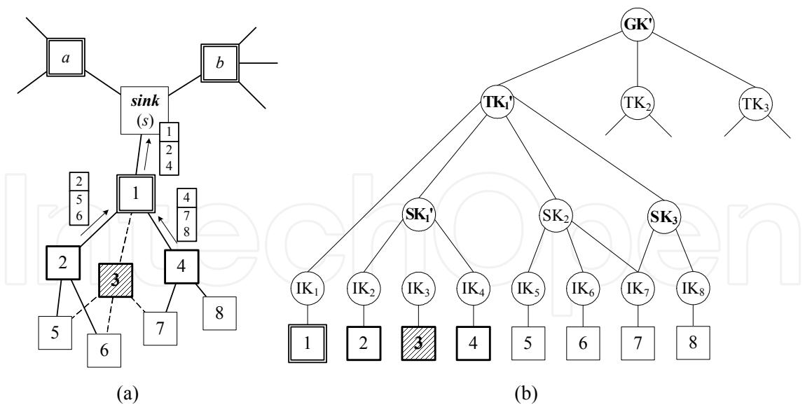
Fig. 9. After non-leaf node 3 in Figure 7 is revoked, a) the repaired routing tree with the re-learning procedure and b) the modified key tree structure.
