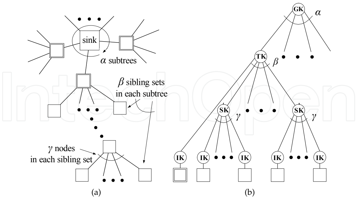
Fig. 10. (a) ‘ \alpha\beta\gamma -tree’ and (b) the corresponding TKH key tree structure.
