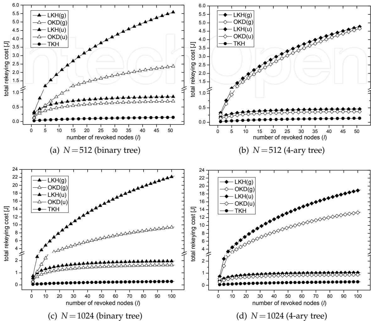
Fig. 15. Simulation results of totla rekeying costs according to increasing number of revoked nodes ( l ) when N = 512, 1024 .
