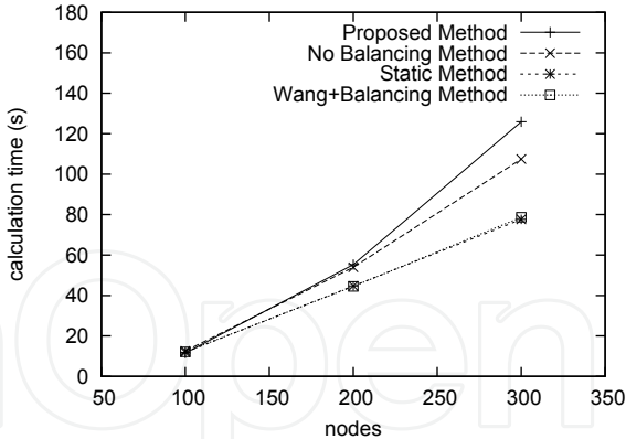
Fig. 6. 3-coverage computation time
