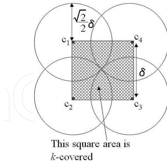
Fig. 4. Checking k -coverage by delta- k -coverage
