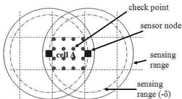
Fig. 7. Example of Misjudge by Wang's Method
