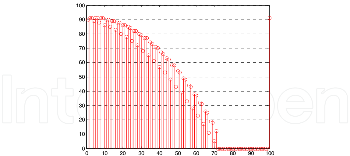
Fig. 4. Number of cycles for each NM in a 3x33star
