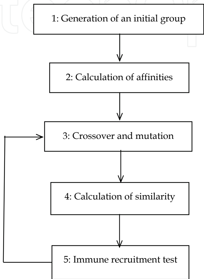
Fig. 3. The GIRM algorithm
