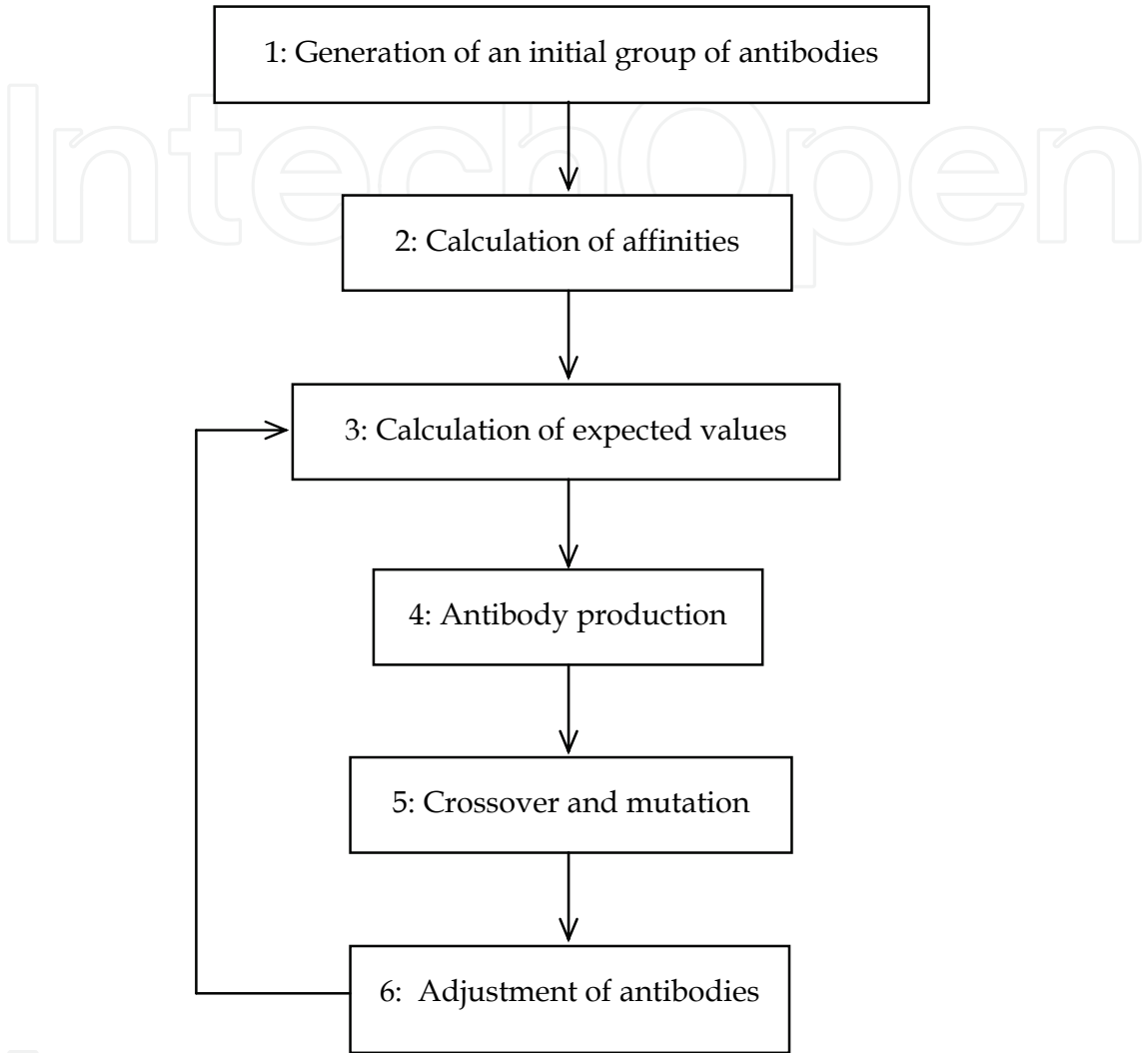
Fig. 1. The GAIAM algorithm
