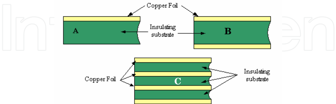
Fig. 2. Three types of PCB structure, (a) Single-sided, (b) Double sided and (c) Multilayer The laminate is then placed into the etching solution and all exposed copper is removed leaving only the desired conductive tracks, the plating in the holes and the lands around the holes (Pardee & Pennino 1988). Once the interconnecting pattern has been created the next phase is to mount and connect the electrical components and thereby assemble the finished board. Small light components may be attached to the board on the surface (surface mounted) (Figure 3) while larger components can be mounted using predrilled holes in the substrate, (through hole) (Figure 4).
