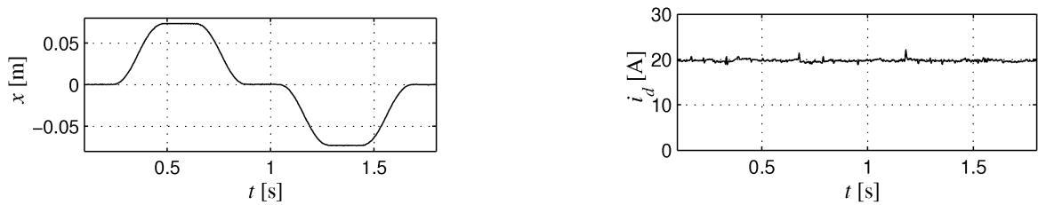
Fig. 11. Trajectories of position x and current i_d measured on the experimental system in the case of kinematic control
