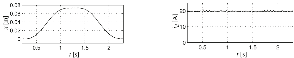
Fig. 13. Trajectories of position x and current i_d measured on the experimental system in the case of low speed kinematic control
