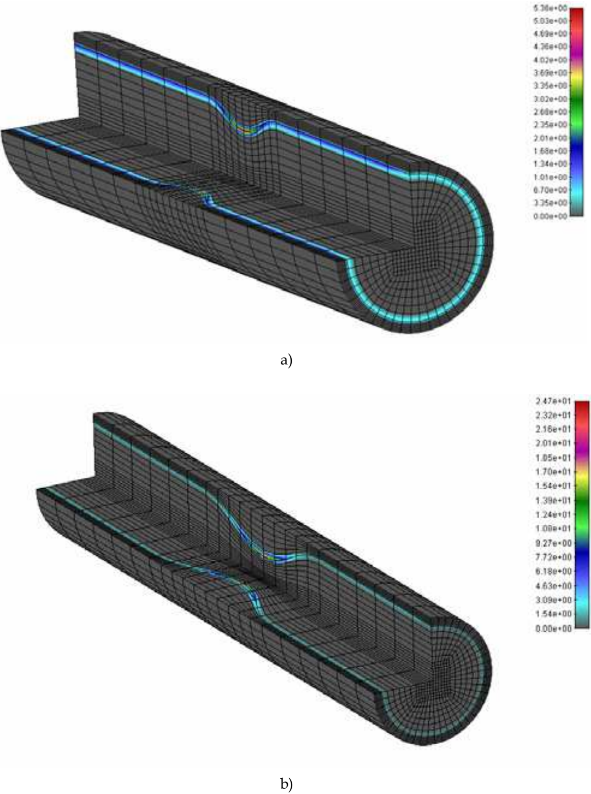
Fig. 13. a) Shear stress distribution for an initial mild stenosis 30% constriction by area b) Shear stress distribution at the end of stenosis process after 10^7 sec[unitsdyn/cm 2 ]
