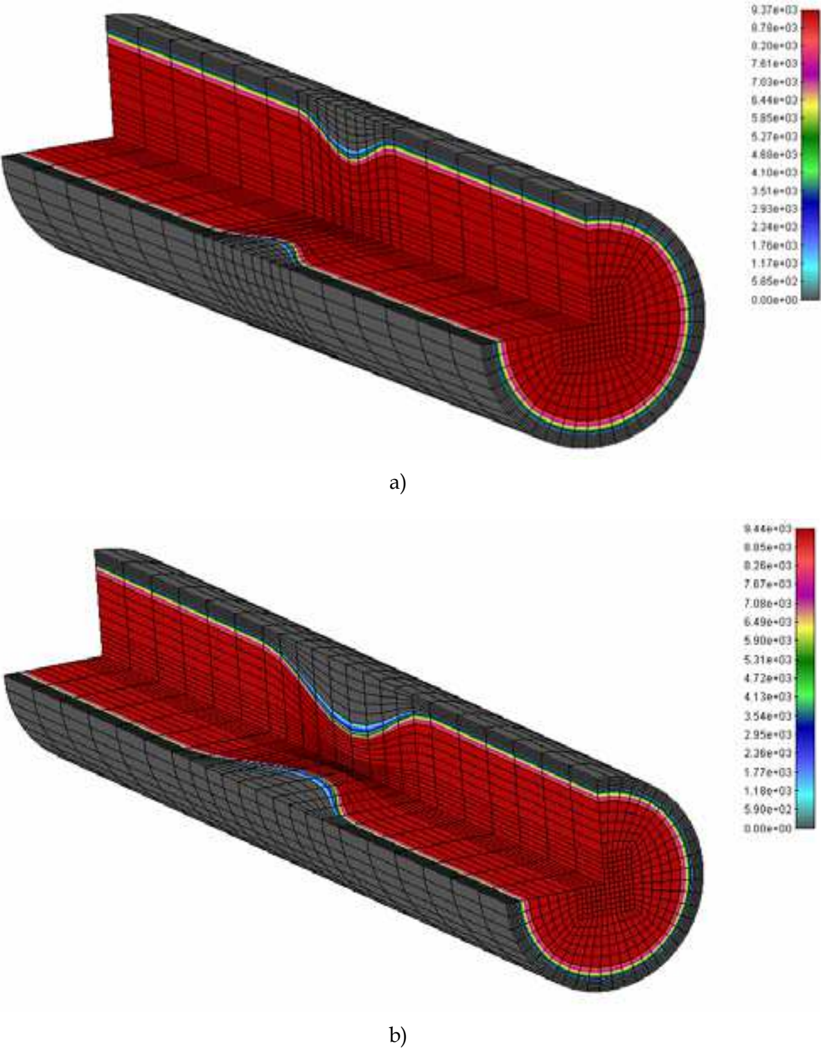
Fig. 12. a) Pressure distribution for an initial mild stenosis 30% constriction by area b) Pressure distribution at the end of stenosis process after 10^7 sec[units Pa]
