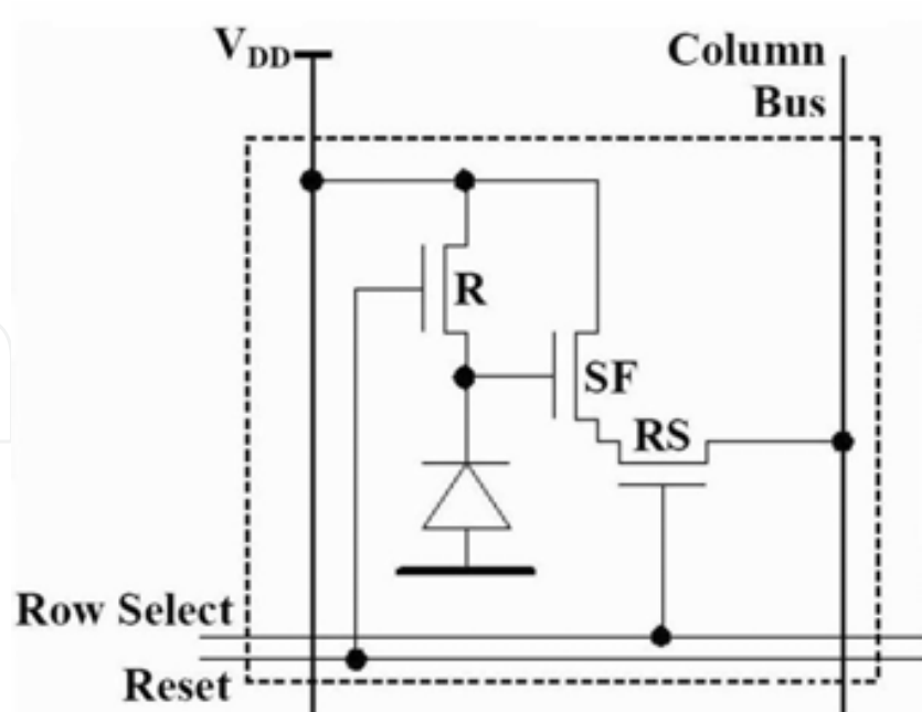
Fig. 2. Three transistor readout for a matrix of pixels. Reset transistor R clears the pixel of integrated charge, Source Follow transistor SF amplifies/buffers the signal and Row Select transistor RS selects the row for readout.
