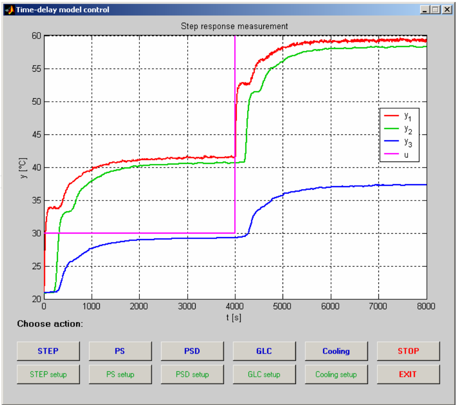
Fig. 17. Heating plant model control application for Matlab 6.5
