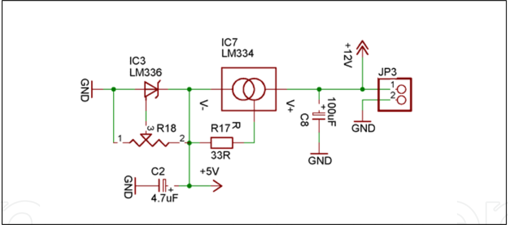
Fig. 6. Power supply for A/D converter schematics
