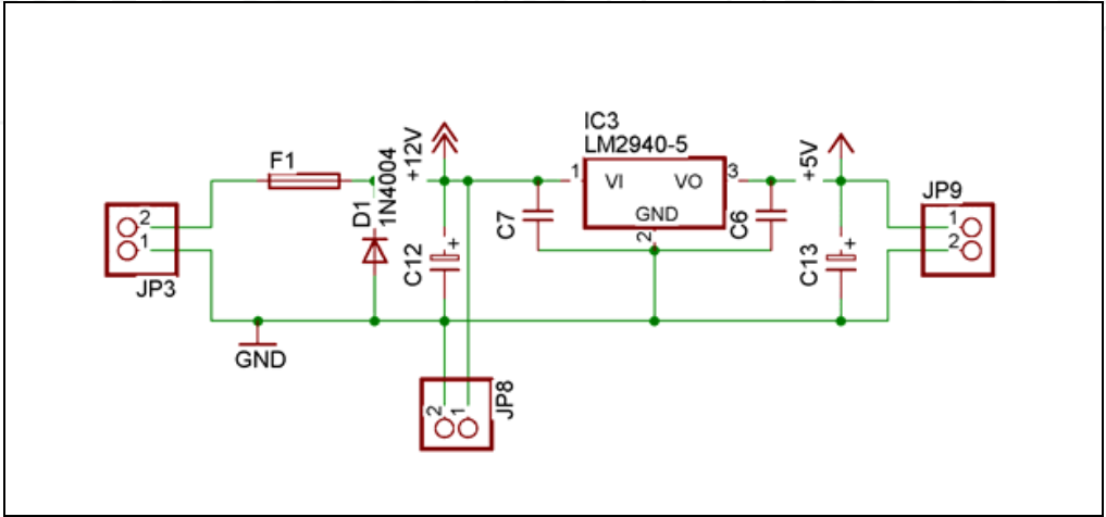
Fig. 5. Power supply for digital circuits schematic
