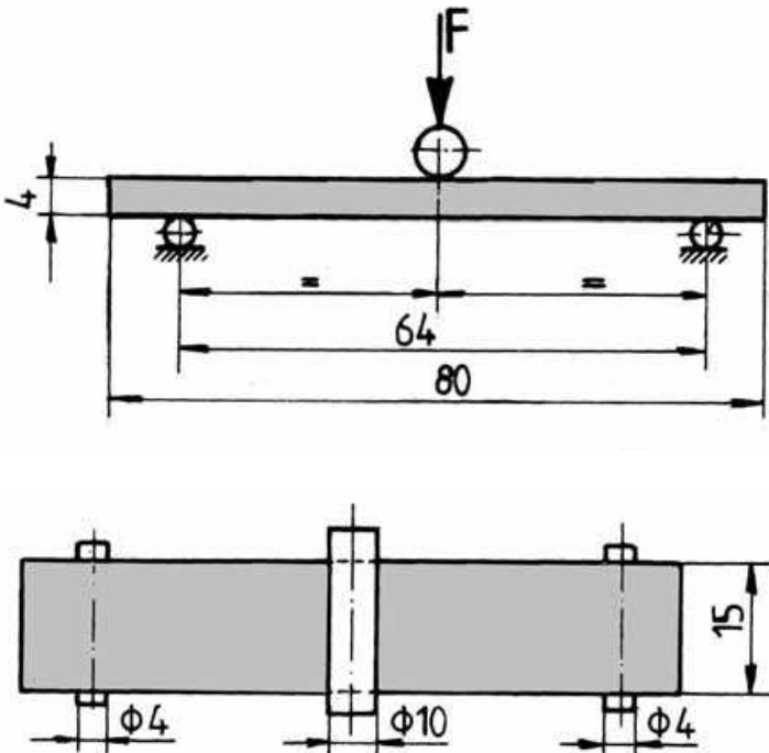
Fig. 3. Specimen used in flexural test
