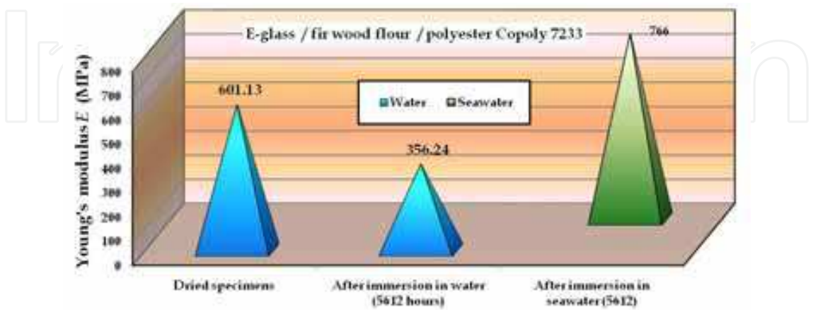
Fig. 28. The effects of water /seawater absorption on Young's modulus E in case of E-glass EWR145 / fir wood flour / polyester Colpoly 7233
