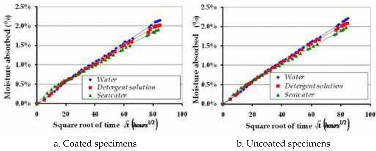
Fig. 8. Absorption data in case of E-glass / epoxy LY 554 composite material
