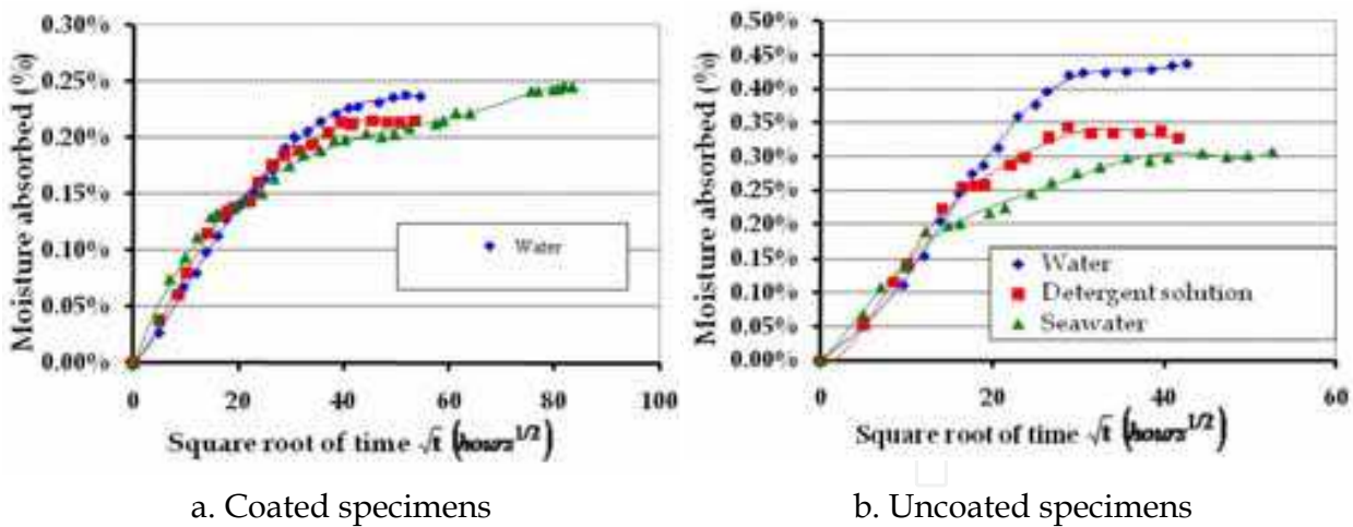
Fig. 9. Absorption data in case of E-glass / vinyl-ester Atlac 582 composite The absorption curves recorded in case of the two hybriide composites are drawn in the figure 10 in case of the immersion in water and in the figure 11 in case of the immersion in seawater.
