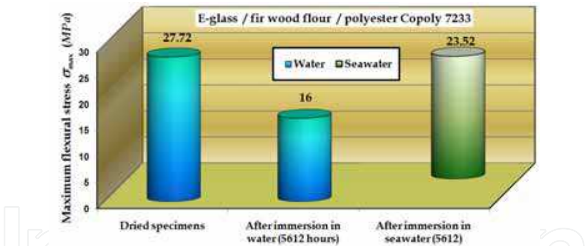
Fig. 29. The effects of water /seawater absorption on on the maximum flexural stress \sigma_{\max} in case of E-glass EWR145 / fir wood flour / polyester Colpoly 7233
