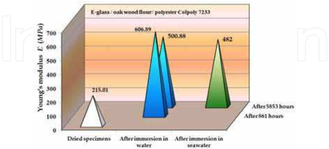
Fig. 30. The effects of water /seawater absorption on Young's modulus E in case of E-glass EWR145 / oak wood flour / polyester Colpoly 7233
