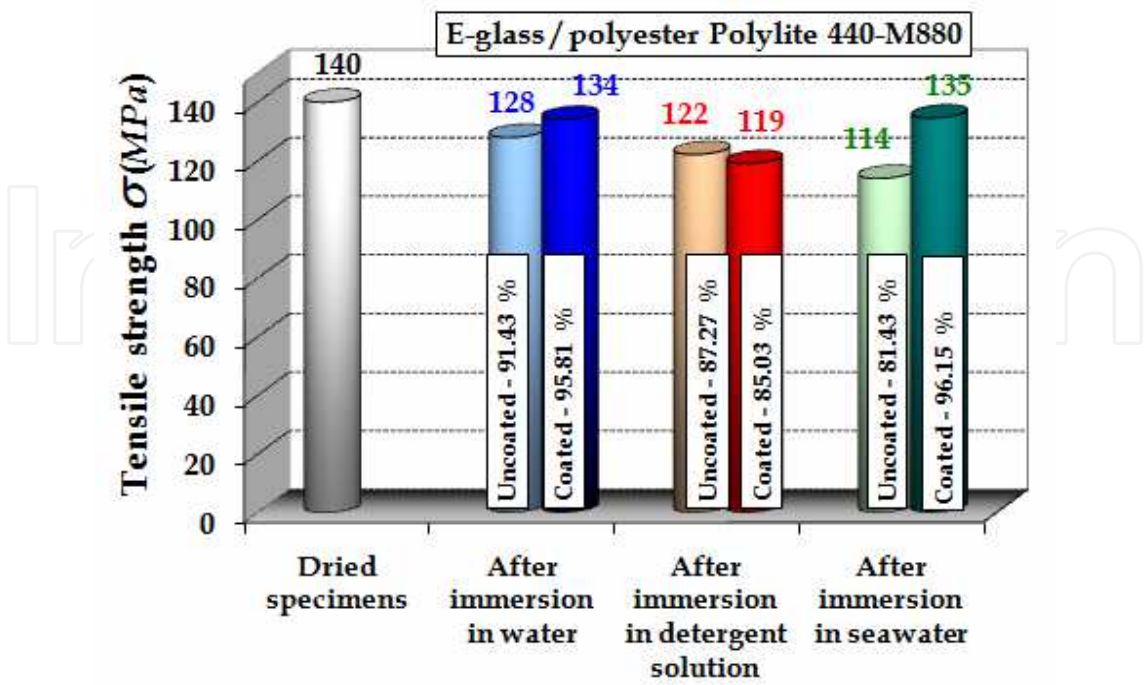
Fig. 14. Changes of the tensile strength in case of E-glass / Polylite 440-M880 composite
