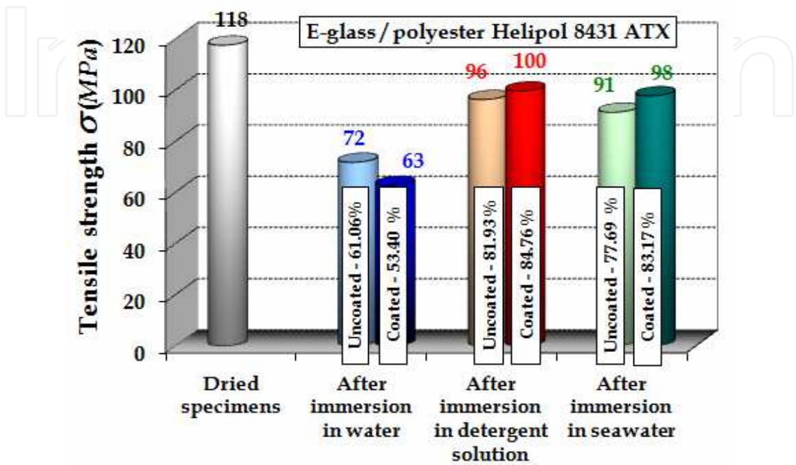
Fig. 13. Changes of the tensile strength in case of E-glass / Heliopol 8431 ATX composite
