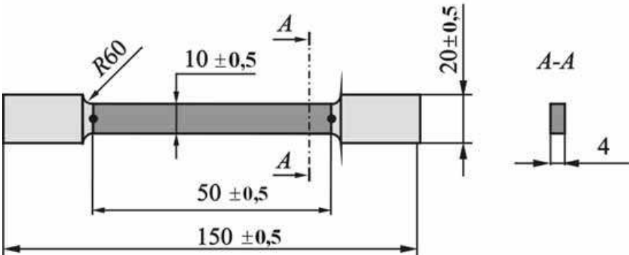
Fig. 2. Specimen for tensile test
