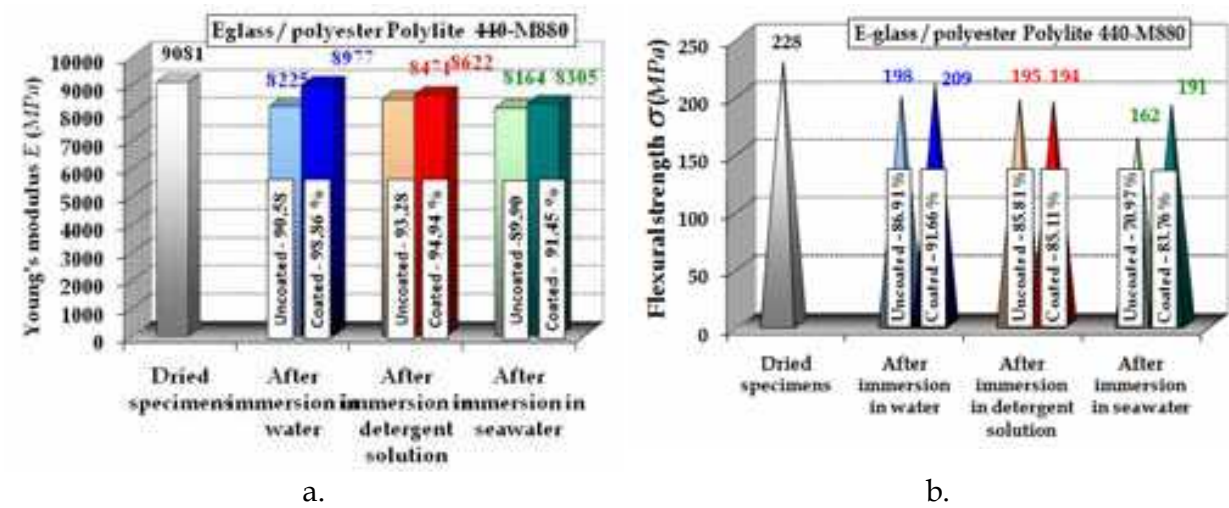
Fig. 25. Experimental results of the flexural test in case of E-glass / PolyLite 440-M880 composite
