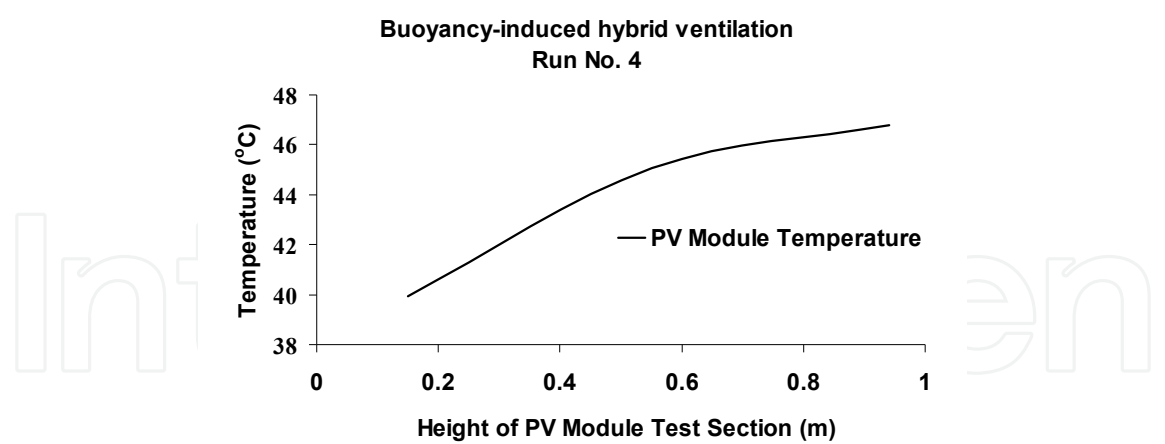
Fig. 6.(a) Temperature plot of PV module for buoyancy-induced hybrid ventilation with height of PV module test section
