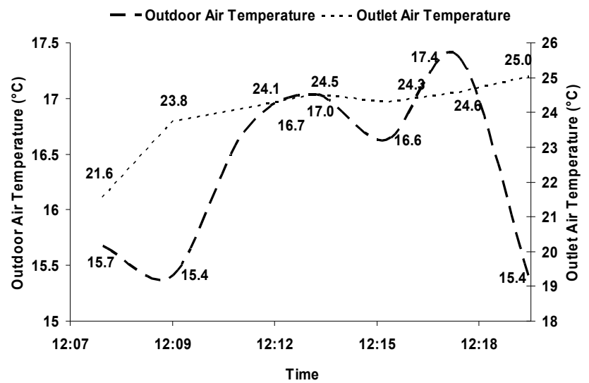
Fig. 10.(b) Changes in outlet air temperature from PV module test section with a step change in outdoor air temperature under fan-induced hybrid ventilation
