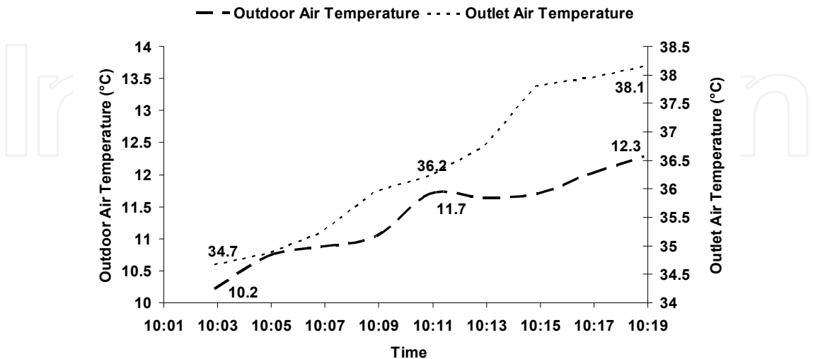
Fig. 10.(a) Changes in outlet air temperature from PV module test section with a step change in outdoor air temperature under buoyancy-induced hybrid ventilation
