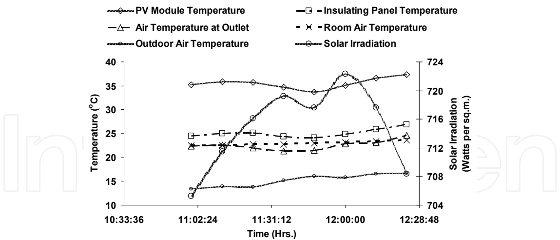
Fig. 7. Variation of mean temperatures of PV module, air and insulating panel with solar irradiation under fan-induced hybrid ventilation
