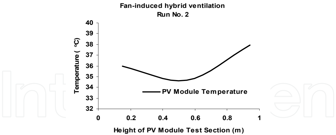
Fig. 5.(a) Temperature plot of PV module for fan-induced hybrid ventilation with height of PV module test section
