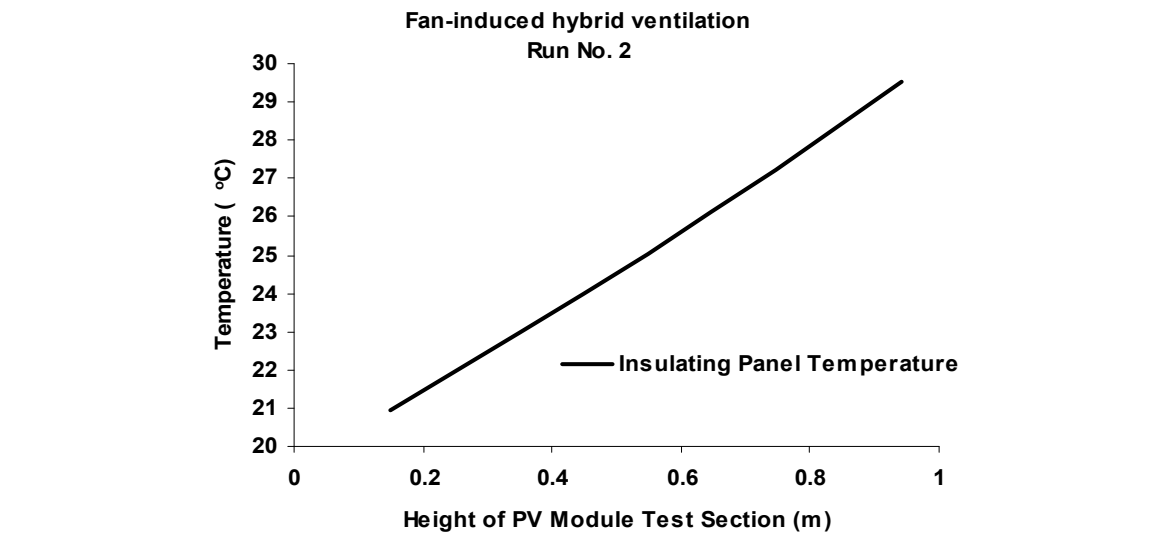
Fig. 5.(b) Temperature plot of insulating panel for fan-induced hybrid ventilation with height of PV module test section
