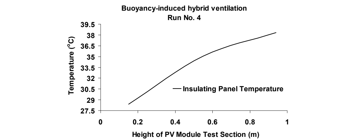
Fig. 6.(b) Temperature plot of insulating panel for buoyancy-induced hybrid ventilation with height of PV module test section
