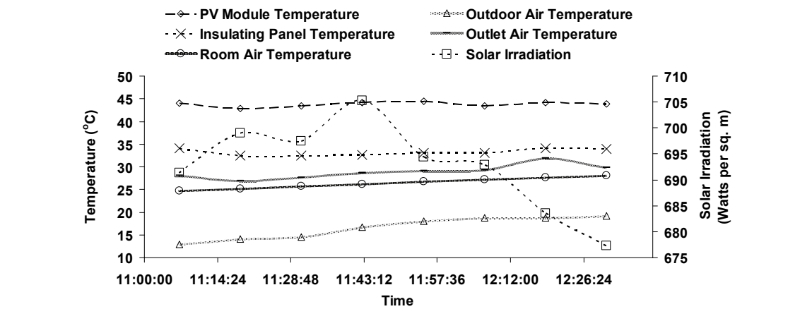
Fig. 8.(a) Variation of mean temperatures of PV module, air and insulating panel with solar irradiation under buoyancy-induced hybrid ventilation
