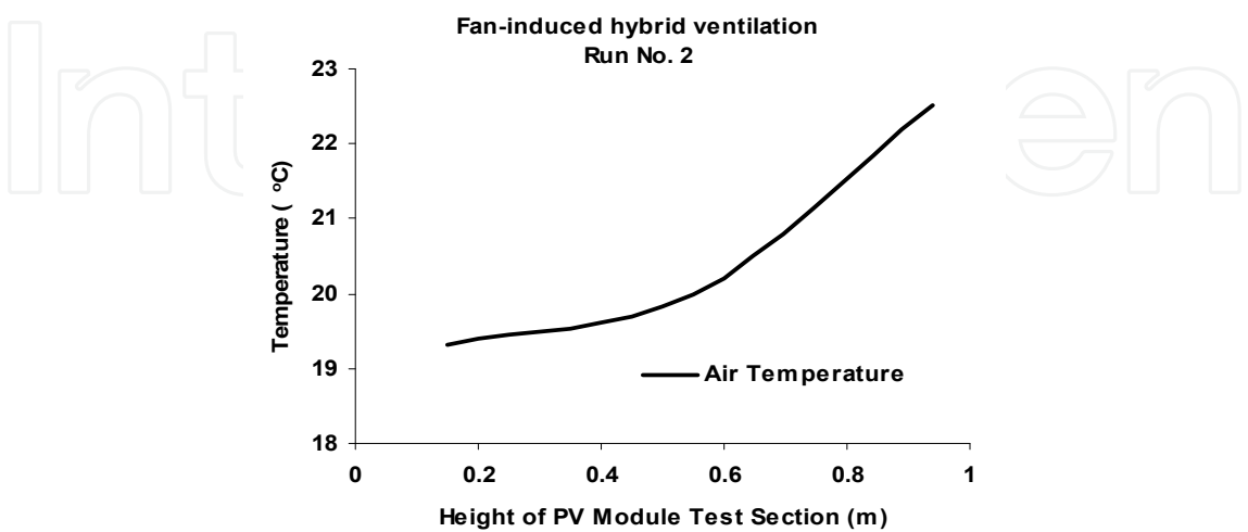
Fig. 5.(c) Temperature plot of air for fan-induced hybrid ventilation with height of PV module test section
