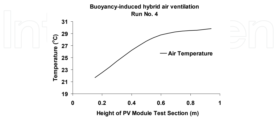
Fig. 6.(c) Temperature plot of air for buoyancy-induced hybrid ventilation with height of PV module test section
