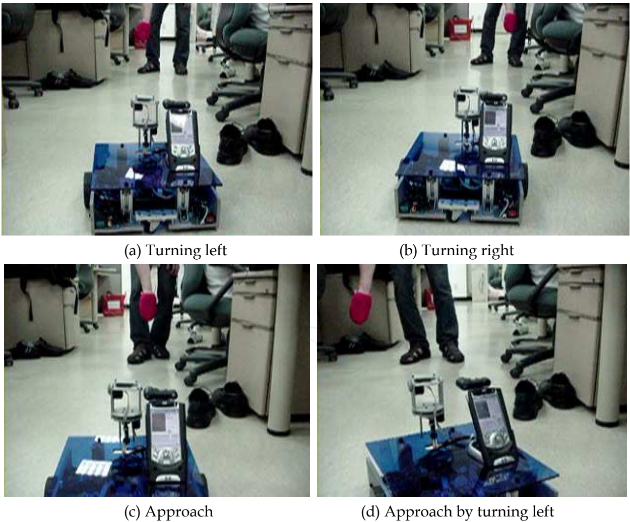
Fig. 18. The experimental results of moving object tracking.
