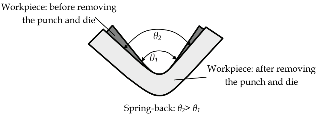
Fig. 9. Illustration of Spring-back Feature
