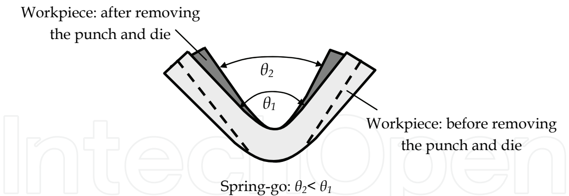
Fig. 10. Illustration of Spring-go Feature
