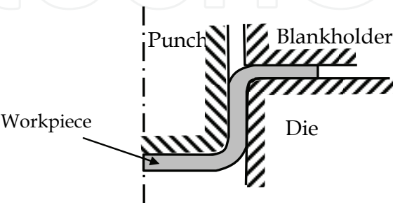
Fig. 2. Bending in deep-drawing process
