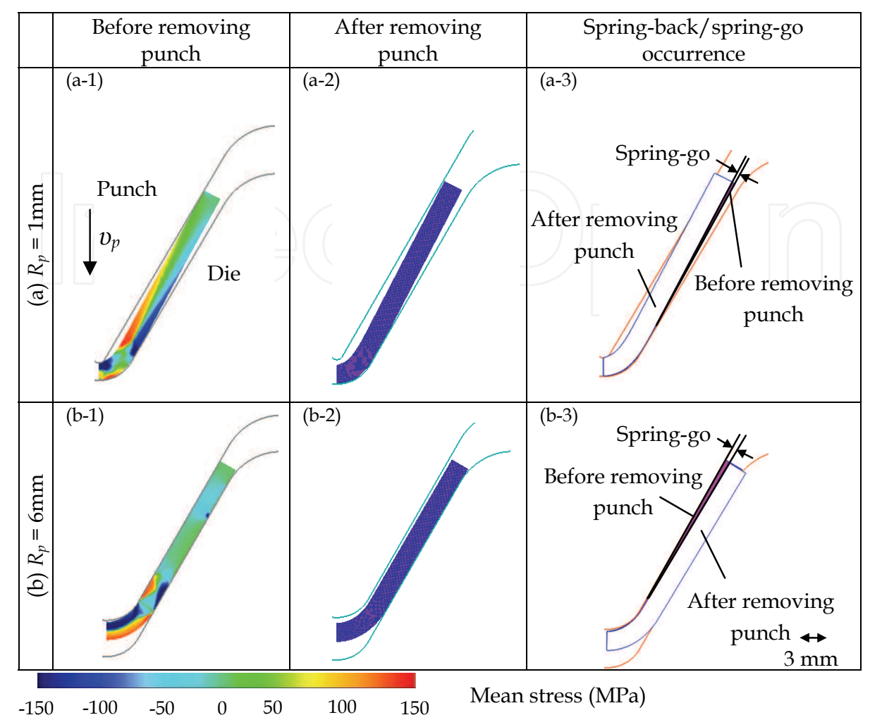
Fig. 14. Characteristics of Spring-back and Spring-go Mechanisms (A1100-O, t = 3\text{ mm} , \theta = 60^\circ , R_d = 6\text{ mm} ) (Thipprakmas & Rojananan, 2008)
