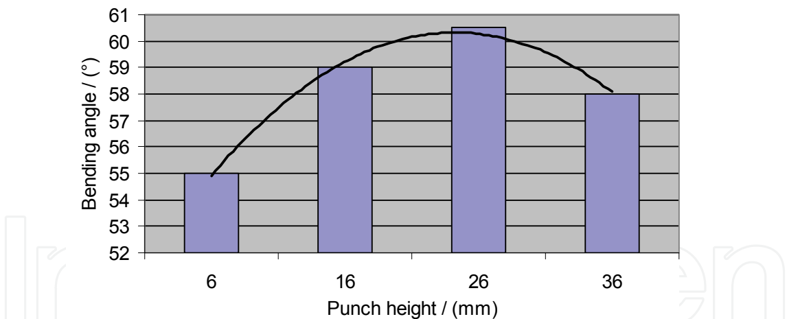
Fig. 19. Bending Angle Analyzed by FEM with Reference to the Punch Height (A1100-O, t=3\text{ mm} , \theta=60^\circ , R_p=4\text{ mm} , R_d=6\text{ mm} ) (Thipprakmas, 2010)
