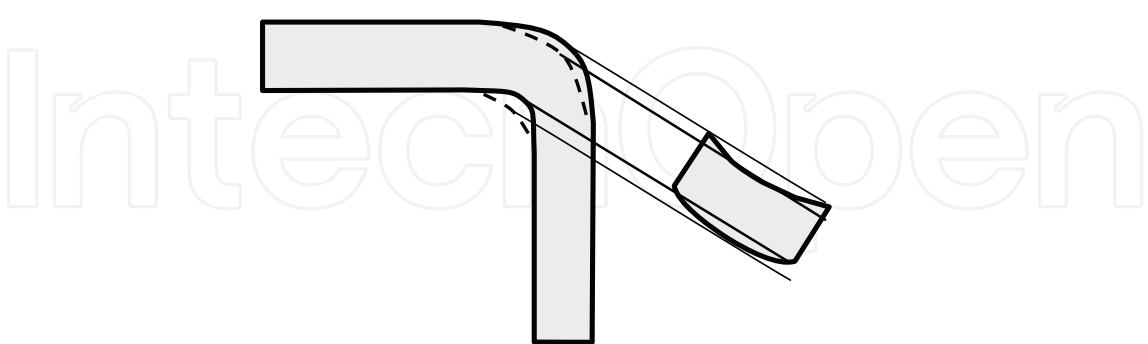
Fig. 7. Unwanted Deformation of the Cross Section during Bending
