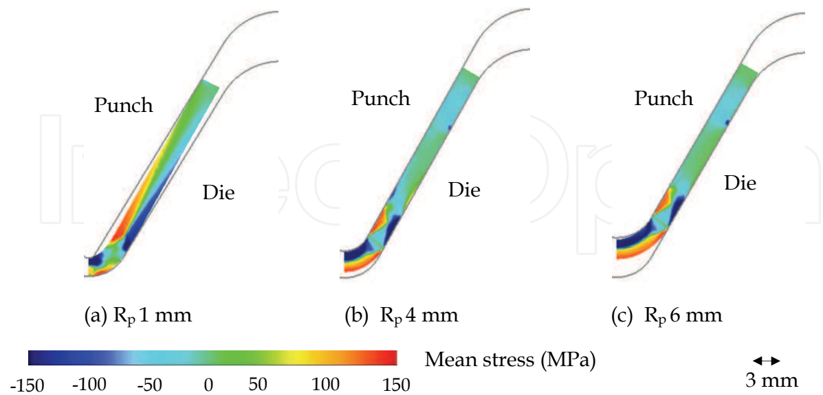
Fig. 16. Stress-Distribution Analysis with Reference to the Punch Radius (A1100-O, t = 3\text{mm} , \theta = 60^\circ , R_d = 6\text{mm} ) (Thipprakmas & Rojananan, 2008)
