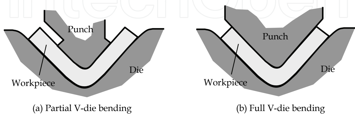
Fig. 6. Classification of the V-die Bending Process
