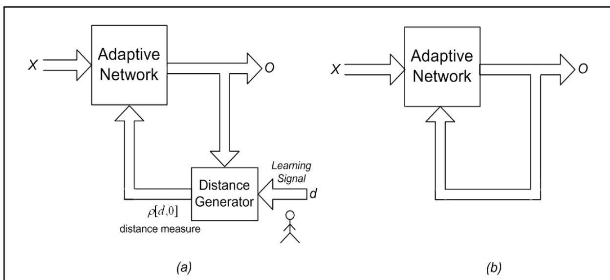
Fig. 6. Basic learning modes
