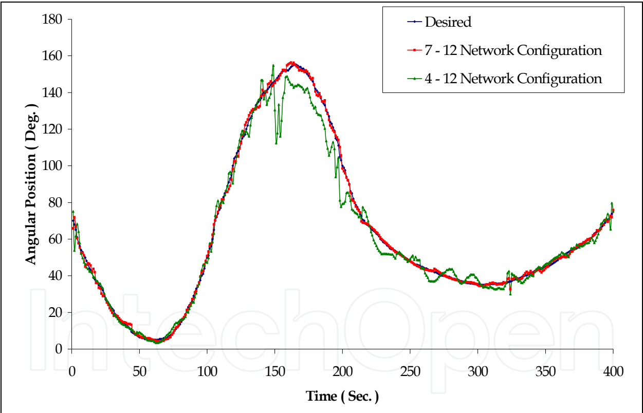
Fig. 10. The response of both network configurations compared to each other during training (The angular position of the firs joint as an example) As a result for the training stage, 7-12 network configuration has shown a better response than the 4-12 network configuration, in terms of precision and iteration (as can be seen through Table 2). Therefore, it has been chosen to apply the testing data. To drive the robot to follow a desired path, it will be necessary to divide this path into small segments, and to move the robot through all intermediate points. To accomplish this task, at each intermediate location, the robot’s trajectory equations are solved, a set of joint variables
