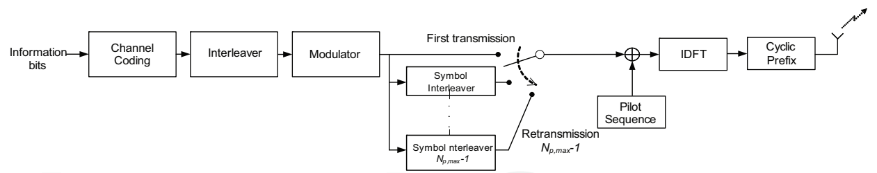
Fig. 2. Emitter Structure
