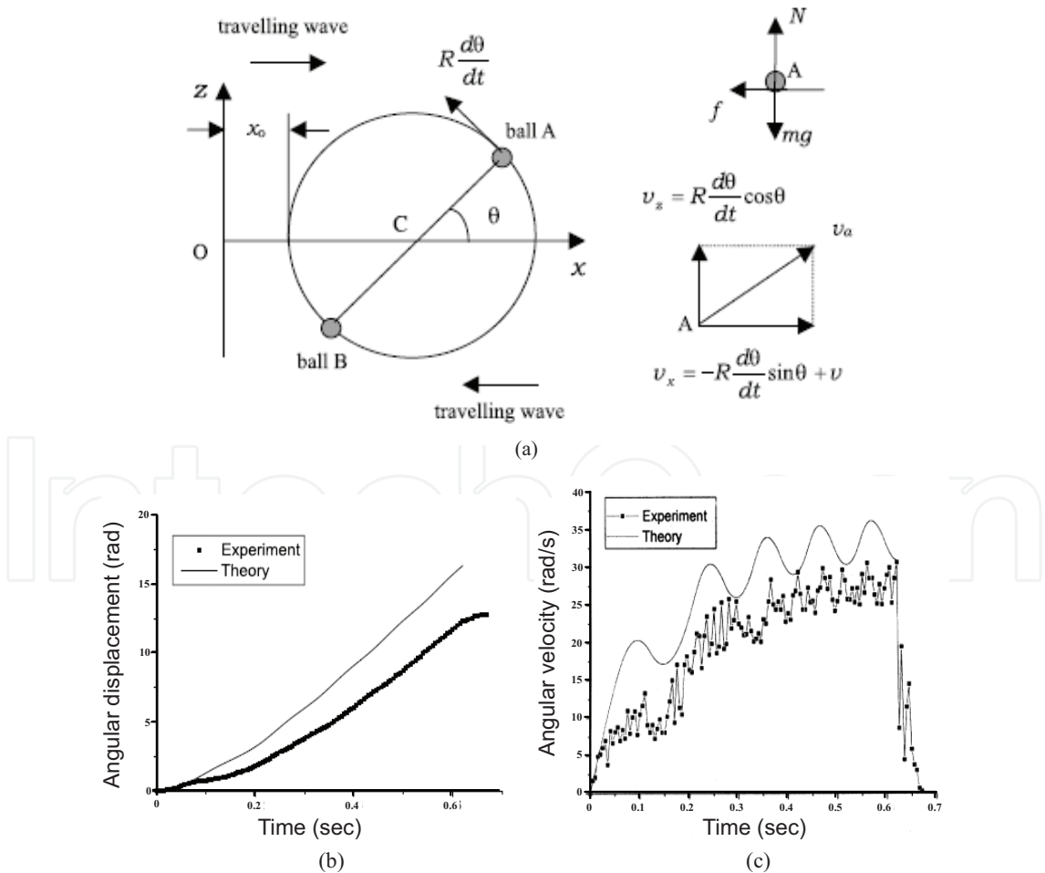
Fig. 9. Numerical simulations of rotary motors: (a) theoretical model; (b) angular displacement versus time; (c) angular velocity versus time.
