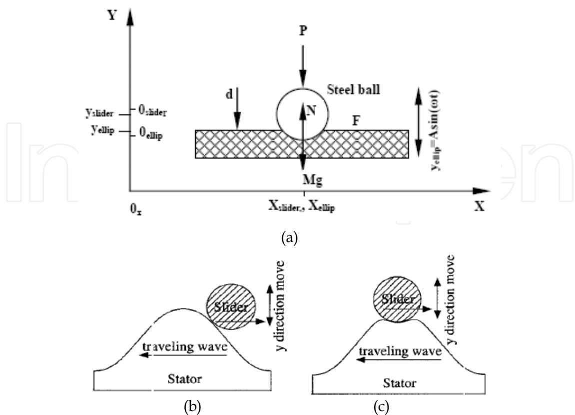
Fig. 7. Theoretical model of SAW linear motor: (a) position of slider; (b) levitation; (c) contact
