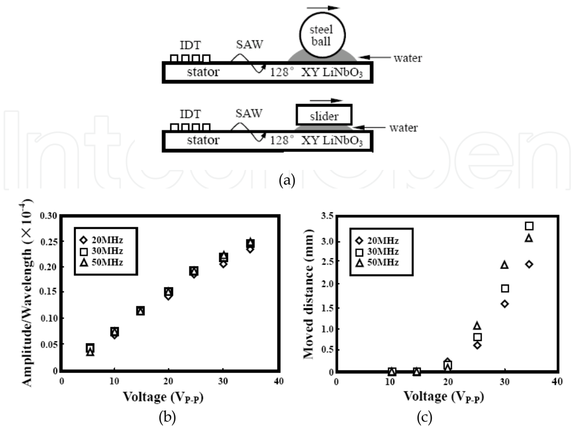
Fig. 11. SAW manipulator: (a) schematic diagram; (b) amplitude/wavelength VS voltage; (c) distance VS voltage.
