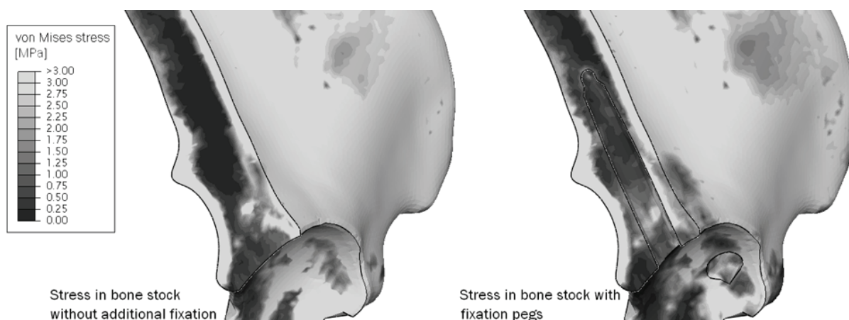
Fig. 12. Cross-sectional view of the von Mises stresses in the posterior ilium under maximum loads during gait. Stress plot with fixation pegs (right) shows higher internal stress in the trabecular bone than calculated without pegs (left).
