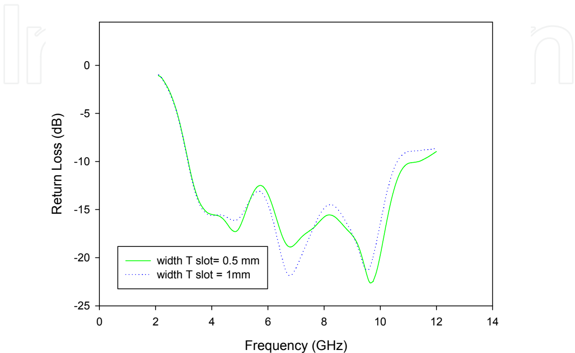
Fig. 12. The simulated return loss for various width of T slots design
