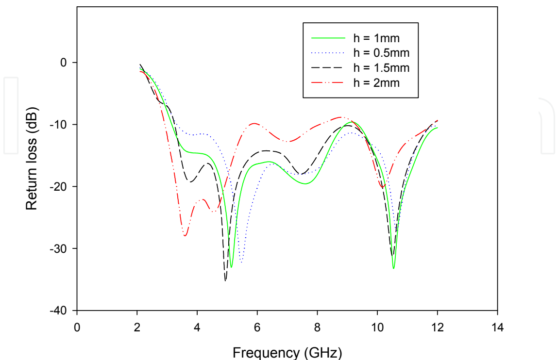
Fig. 4. Simulated return loss curves of T slotted antenna for different feed gaps
