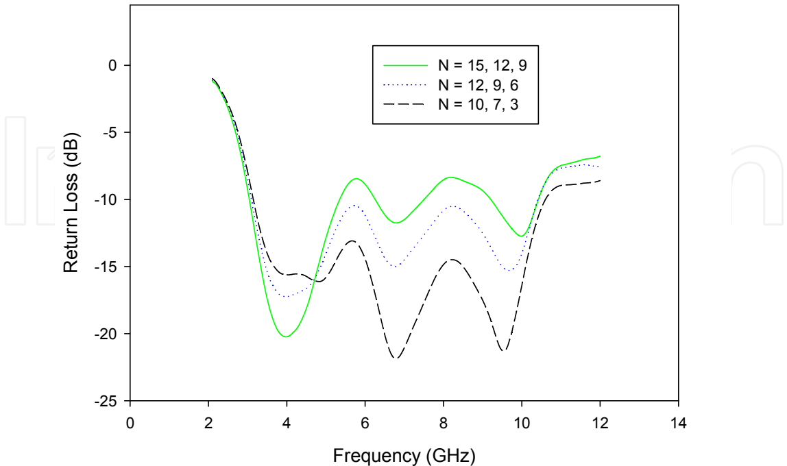
Fig. 7. The effect of various length slotted ground plane to the antenna performance
