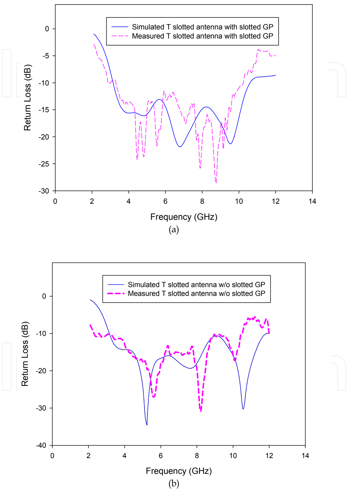
Fig. 14. The measured and simulated return loss for T slotted antenna: (a) with slotted ground plane and (b) without slotted ground plane
