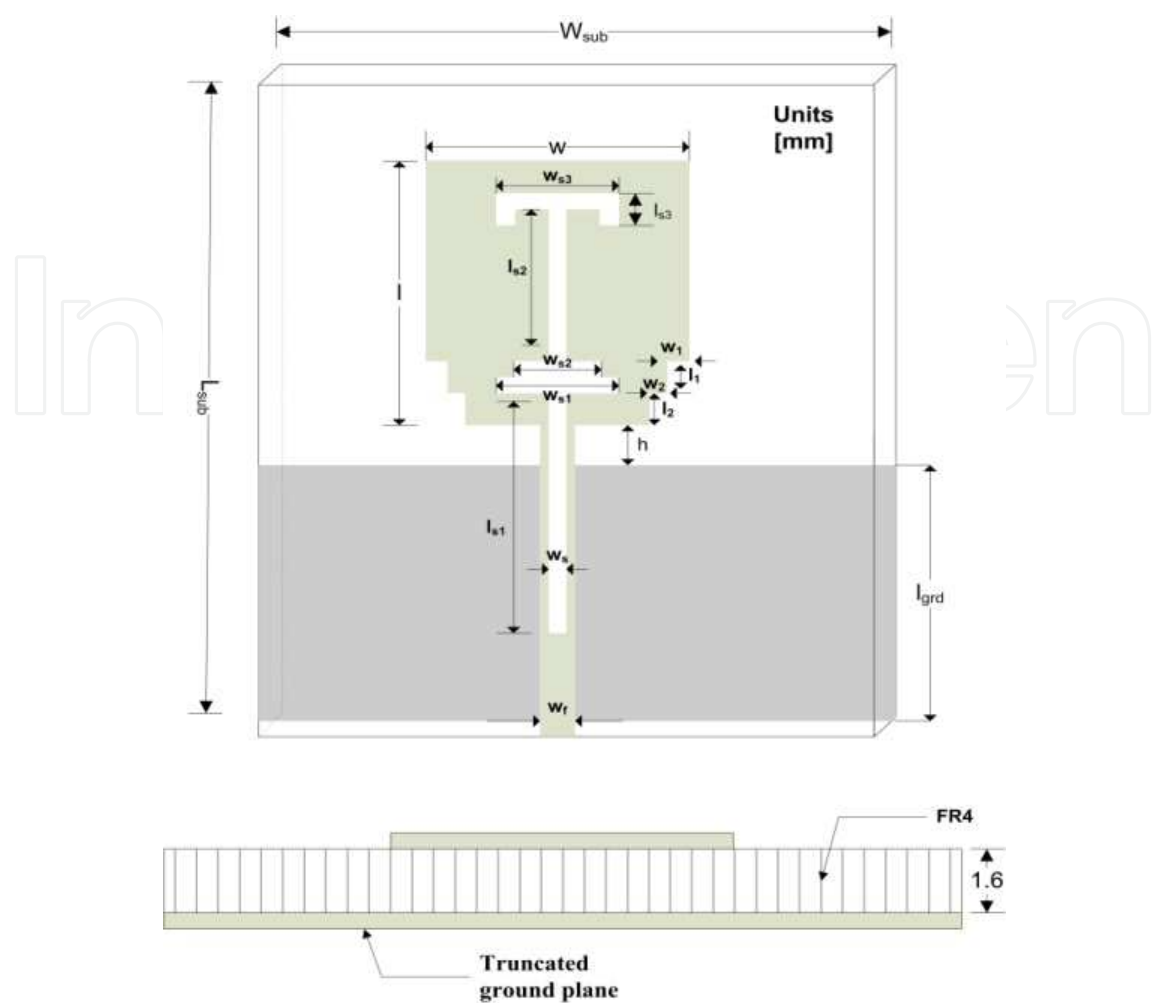
Fig. 1. Geometry of T slotted UWB antenna
