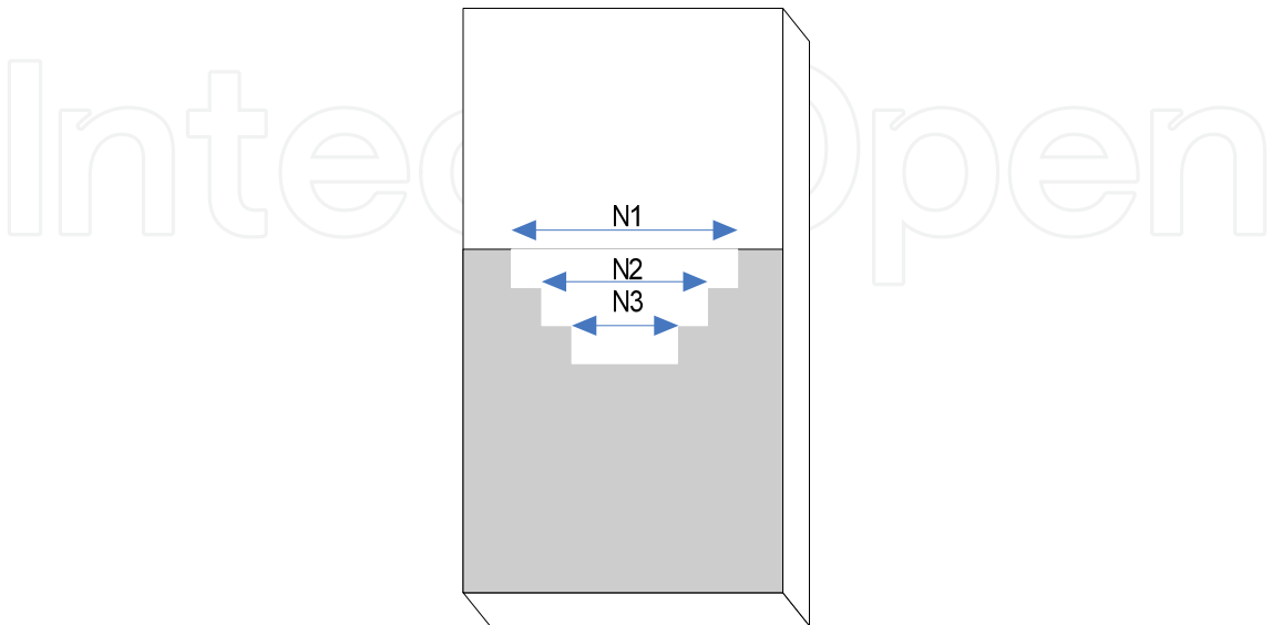
Fig. 6. Geometry of staircase slotted ground plane
