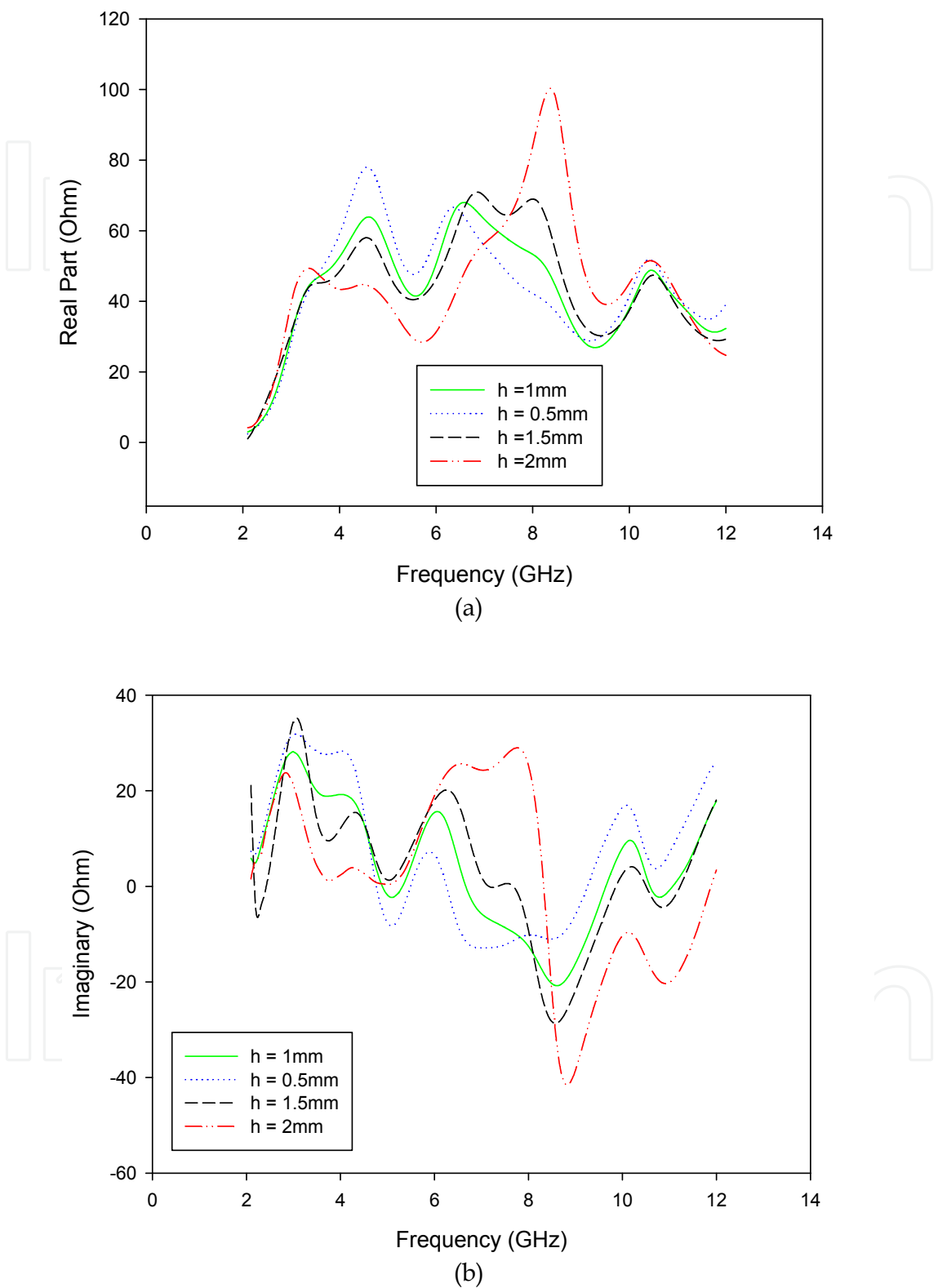
Fig. 5. Simulated input impedance curves of T slotted antenna for different feed gaps: (a) real part and (b) imaginary part
