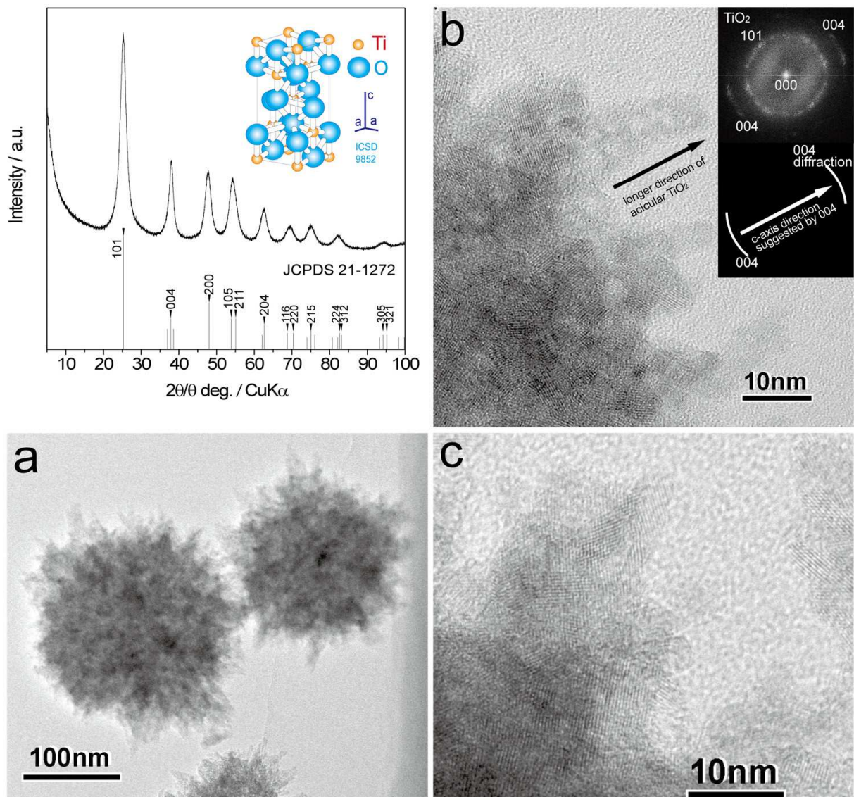
Fig. 4. XRD diffraction pattern of anatase TiO 2 particles. (a): TEM micrograph of anatase TiO 2 particles. (b): Magnified area of (a) showing morphology of acicular crystals. Insertion in (b): FFT image of (b) anatase TiO 2 . (c): Magnified area of (a) showing lattice images of anatase TiO 2 .
