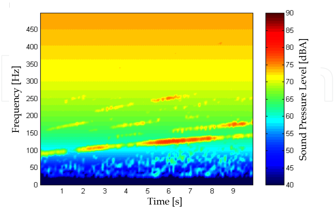
Fig. 13. Order analysis of sound pressure level (passenger’s left ear) of a road test (acceleration from 1800 to 4500 rpm, full throttle, 3rd gear, control on).
