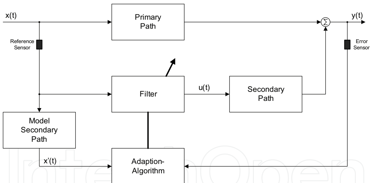
Fig. 4. Block diagram of FxLMS algorithm.
