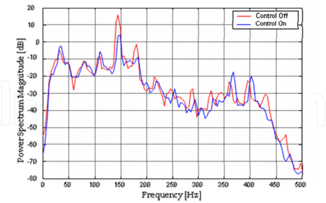
Fig. 14. Power spectrum comparison of the measured steering wheel acceleration for constant drives with 4400 RPM.
