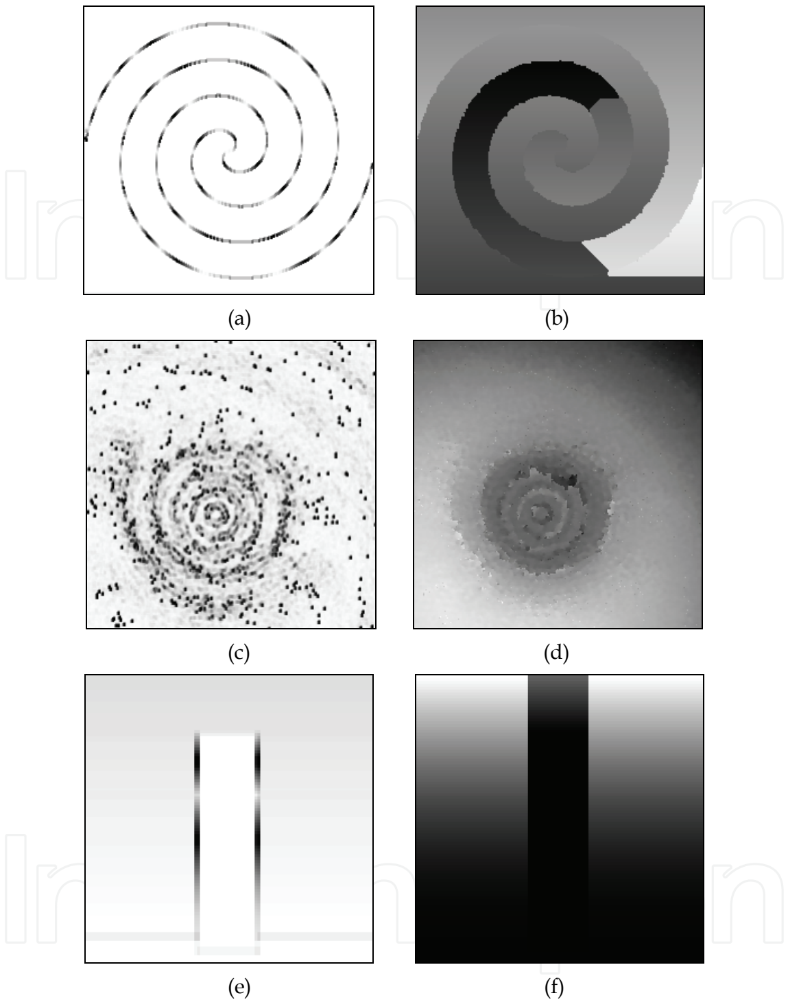
Fig. 5. (a) Maximum phase gradient map of Fig. 1(b). (b) Unwrapping result by use of Fig. 5(a). (c) Maximum phase gradient map of Fig. 1(c). (d) Unwrapping result by use of Fig. 5 (c). (e) Maximum phase gradient map of Fig. 1(e). (f) Unwrapping result by use of Fig. 5 (e).
