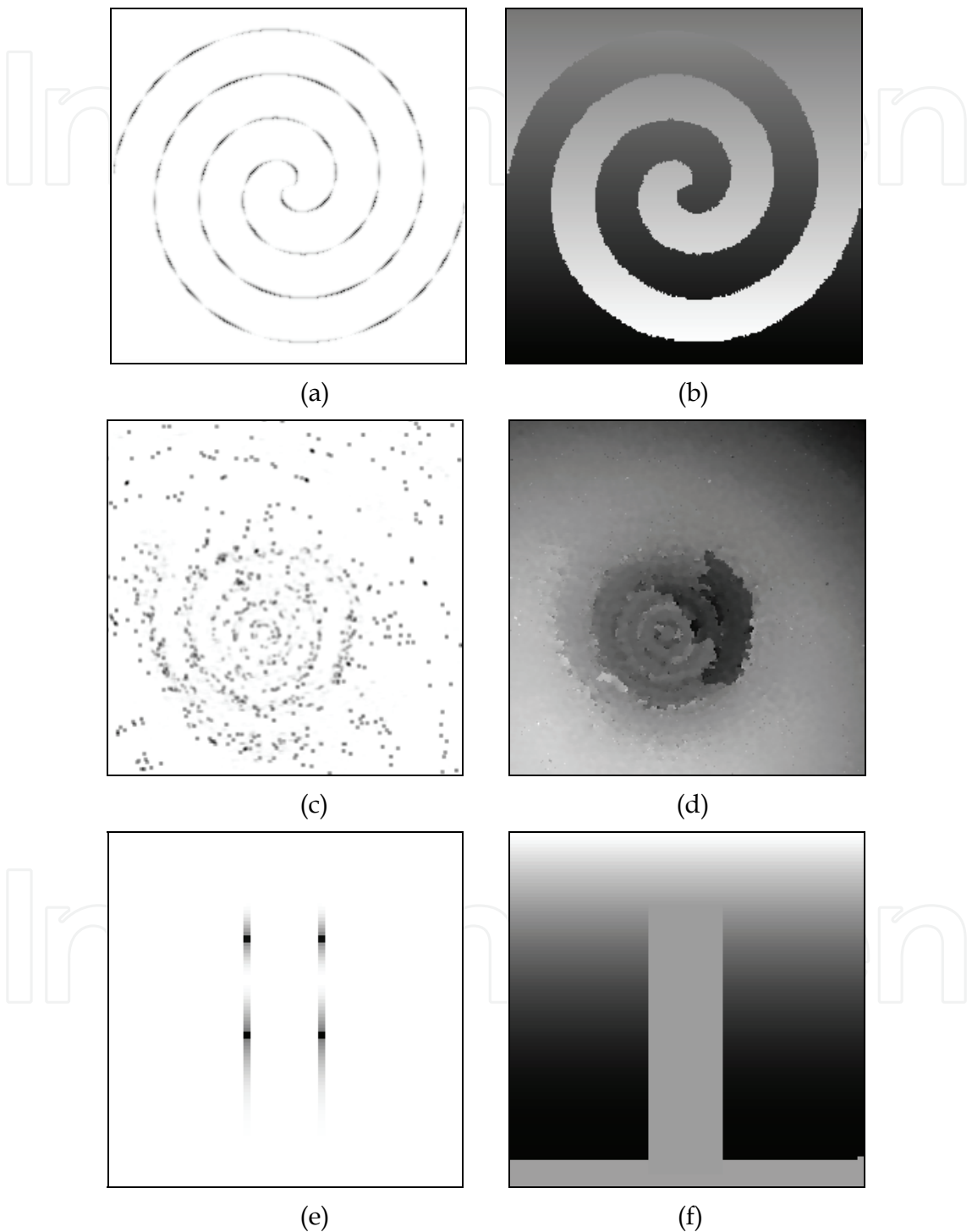
Fig. 4. (a) Phase derivatives variance map of Fig. 1(b). (b) Unwrapping result by use of Fig. 4(a). (c) Phase derivatives variance map of Fig. 1(c). (d) Unwrapping result by use of Fig. 4(c). (e) Phase derivatives variance map of Fig. 1(e). (f). Unwrapping result by use of Fig. 4(e).
