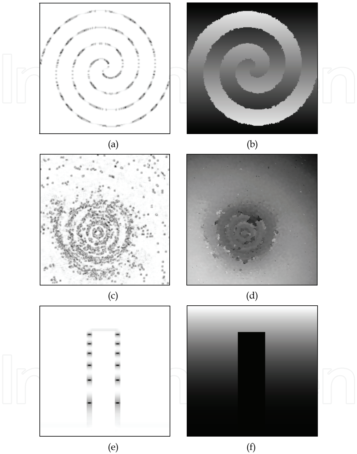
Fig. 9. (a) Weighted phase derivatives variance map of Fig. 1(b) generated by use of Prewitt operators. (b) Unwrapping result by use of Fig. 9(a). (c) Weighted phase derivatives variance map of Fig. 1(c) generated by use of Prewitt operators. (d) Unwrapping result by use of Fig. 9 (c). (e) Weighted phase derivatives variance map of Fig. 1(e) generated by use of Prewitt operators. (f) Unwrapping result by use of Fig. 9(e).
