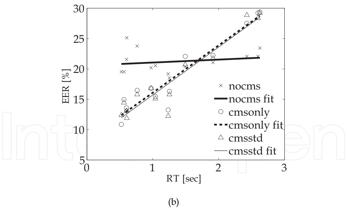
Fig. 5. EER values of SVR with reverberant speech as a function of RT. Cross marks ("x") denote no feature normalization (linear fitting with thick solid line), circles ("o") denote CMS (linear fitting with thick dashed line), and triangles ("Δ") denote using CMS with variance normalization (linear fitting with thin solid line). Test speech segments were made reverberant by convolution with (a) simulated, and (b) measured RIRs.
