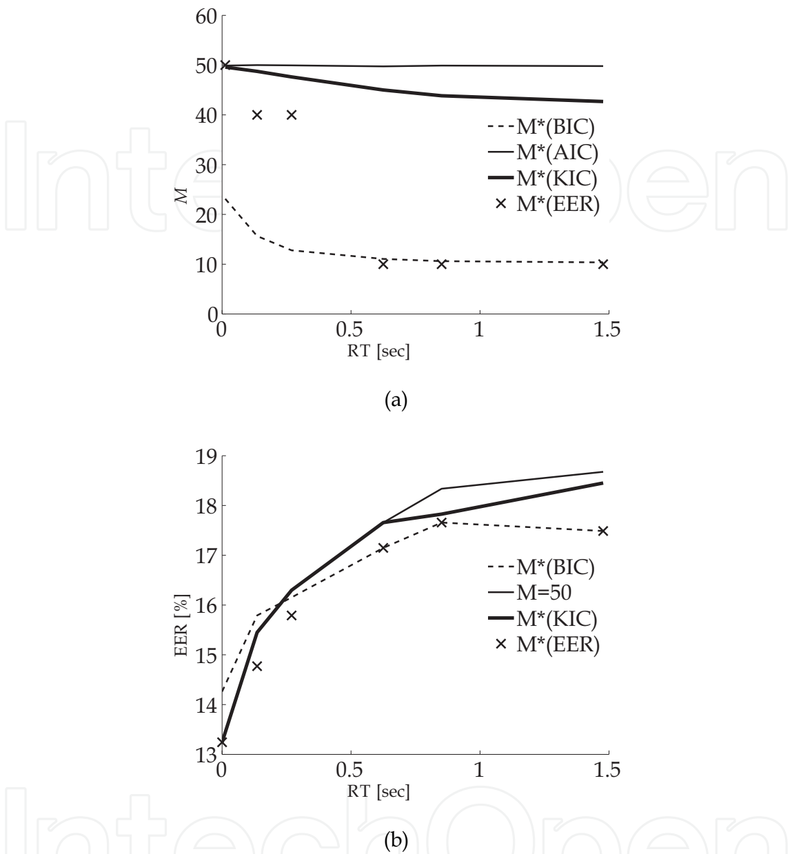
Fig. 4. Comparing results of optimal GMM order using BIC, AIC, and KIC, to the optimal GMM order in terms of minimal EER. (a) Optimal model order, (b) EER values.
