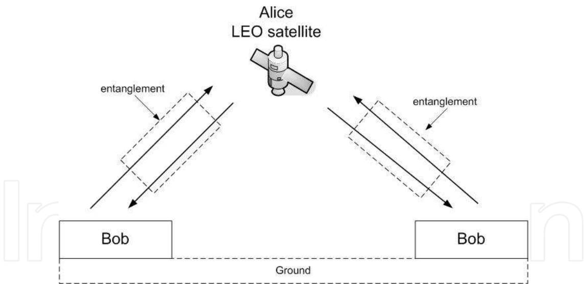
Fig. 7. Satellite-to-ground free-space QKD
