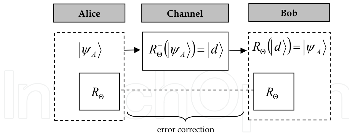
Fig. 10. Redundancy-free error correction, solution 2.
