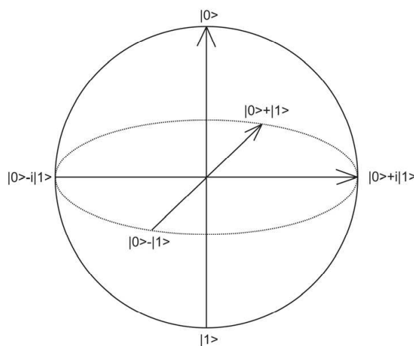
Fig. 2. Bloch sphere – a special visual representation of a quantum bit
