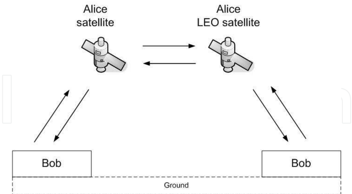
Fig. 6. Global key exchange based free-space QKD
