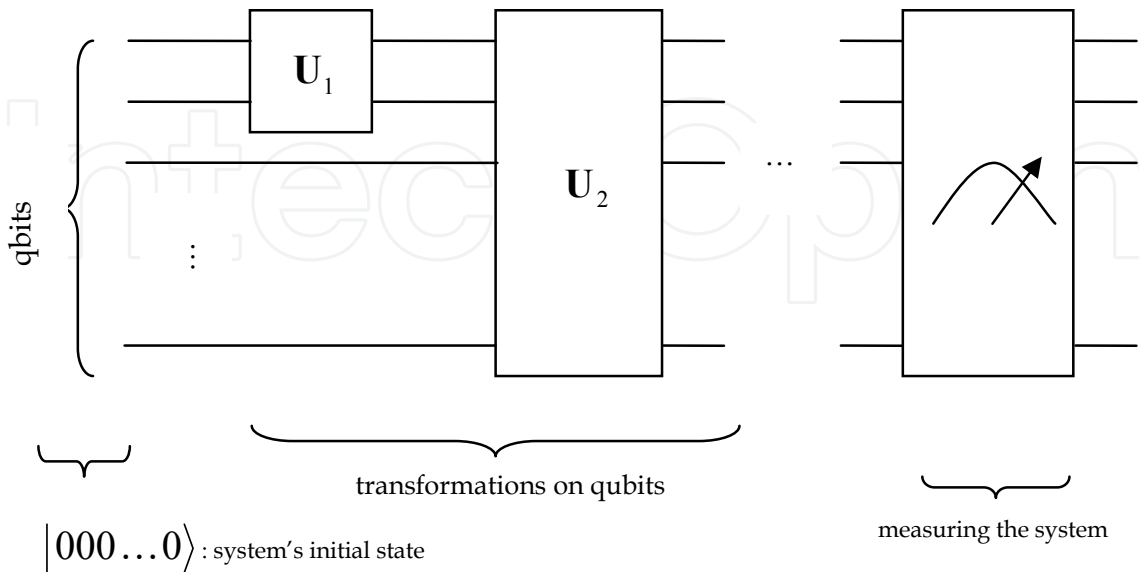
Fig. 3. General model of a quantum circuit
