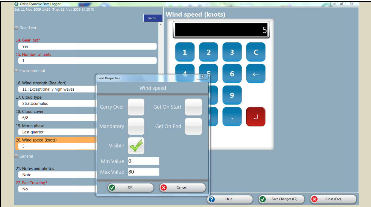
Fig. 9. Olfish-DDL user configuration form
