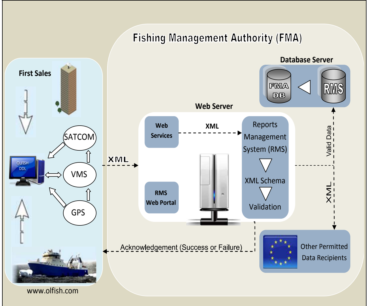
Fig. 1. Overall structure of the Olfish data collection and management system
