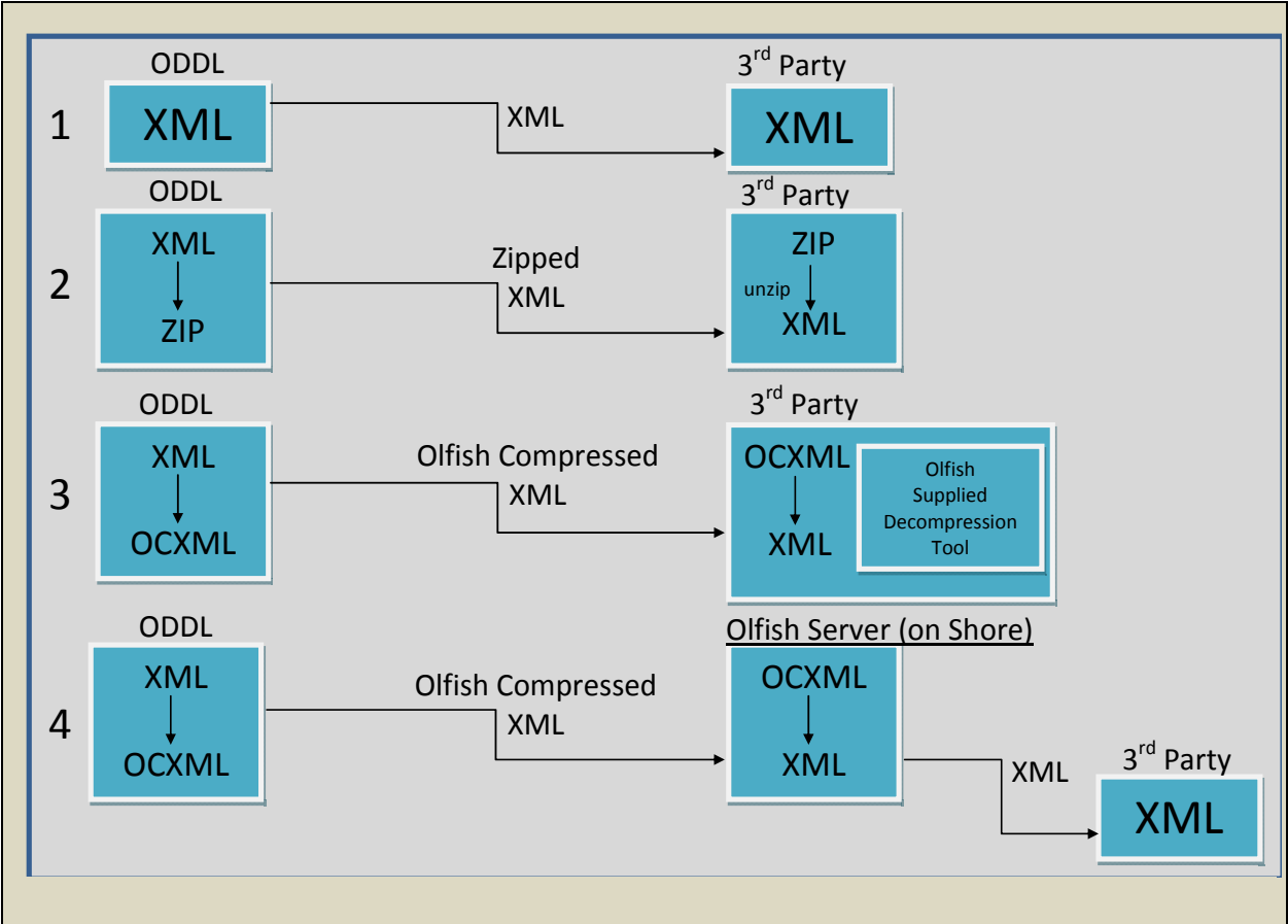
Fig. 13. Transmission of XML files from Olfish- DDL (vessel unit) to third-party (Olfish-DDL shore unit or RMS)
