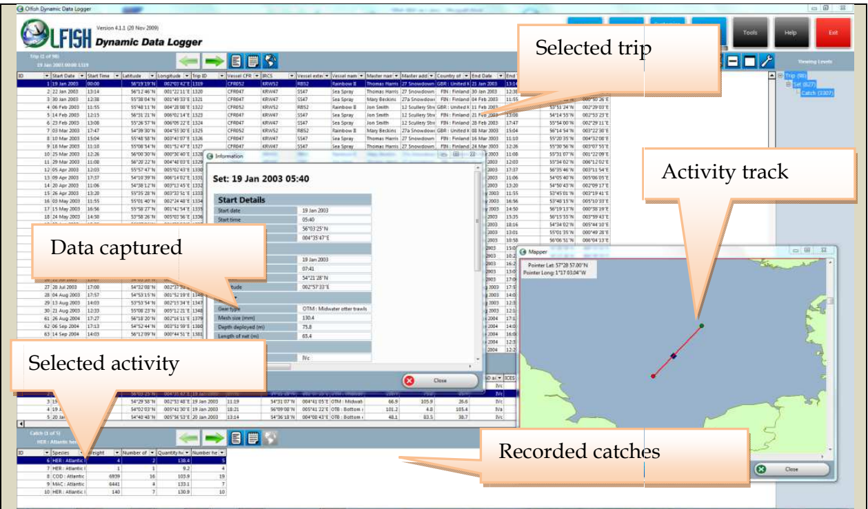
Fig. 8. Olfish-DDL main database interface (Data Centre)
