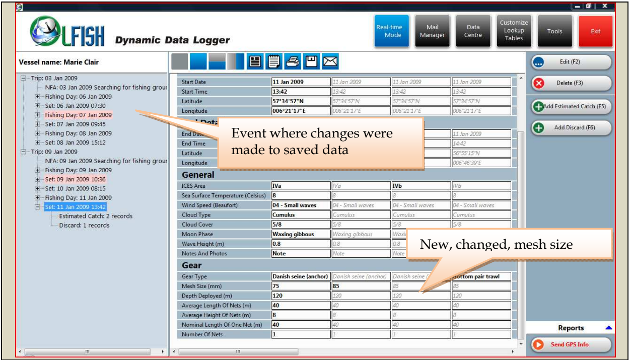
Fig. 14. Change-Control utility: pink markers on the activity tree show places where changes took place, bold figures in 2 nd , 3 rd and 4 th columns were changed.
