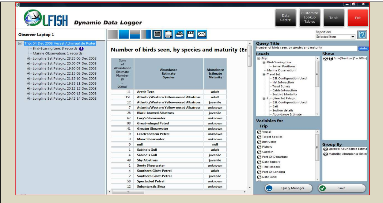
Fig. 17. Mini-Reporter: The HTML browser in the centre is changed to reflect the query output as was set up on the right.
