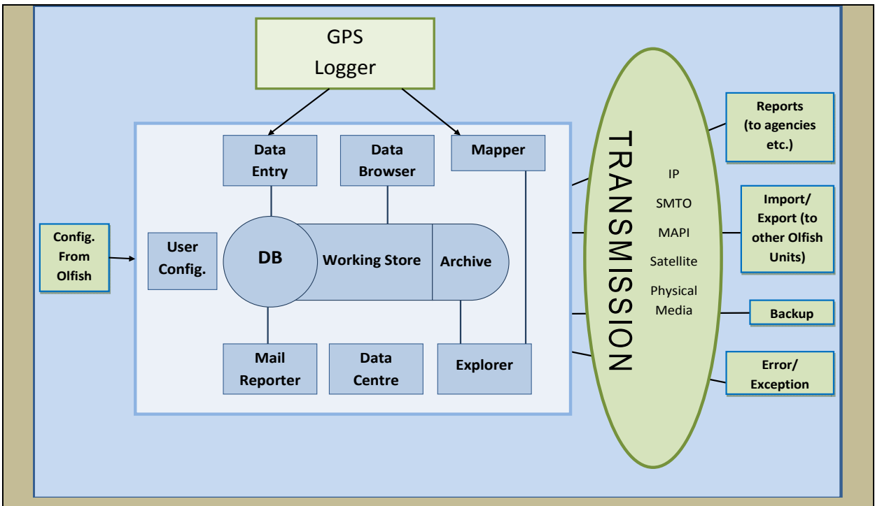
Fig. 3. Olfish-DDL basic structure
