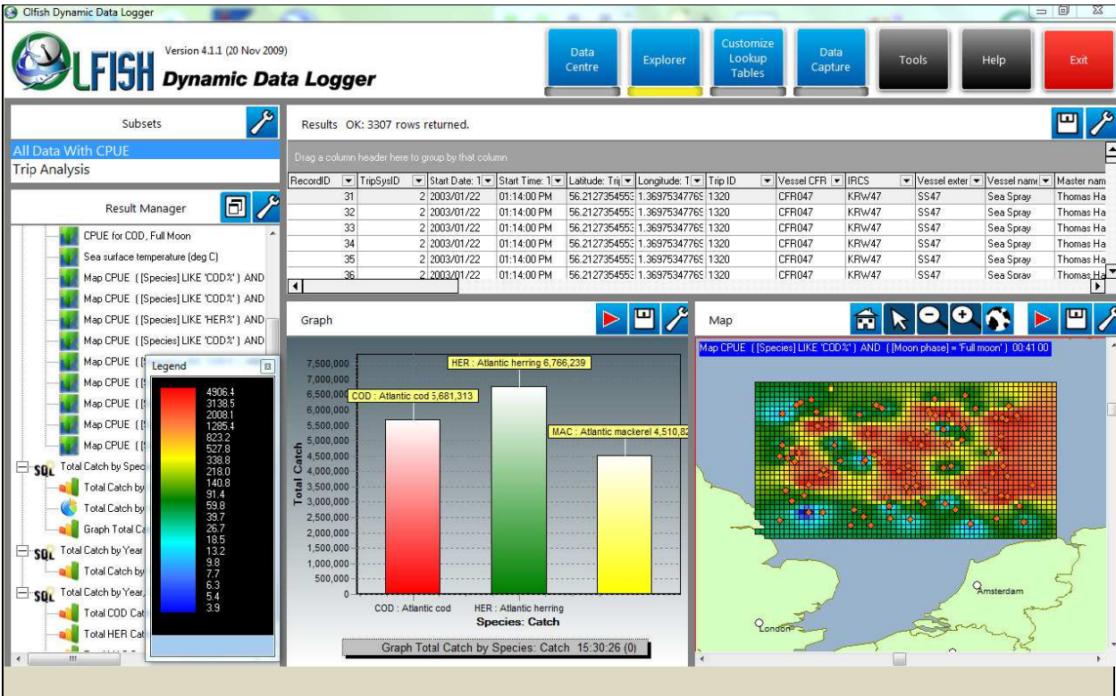
Fig. 18. Olfish-Explorer view mode
