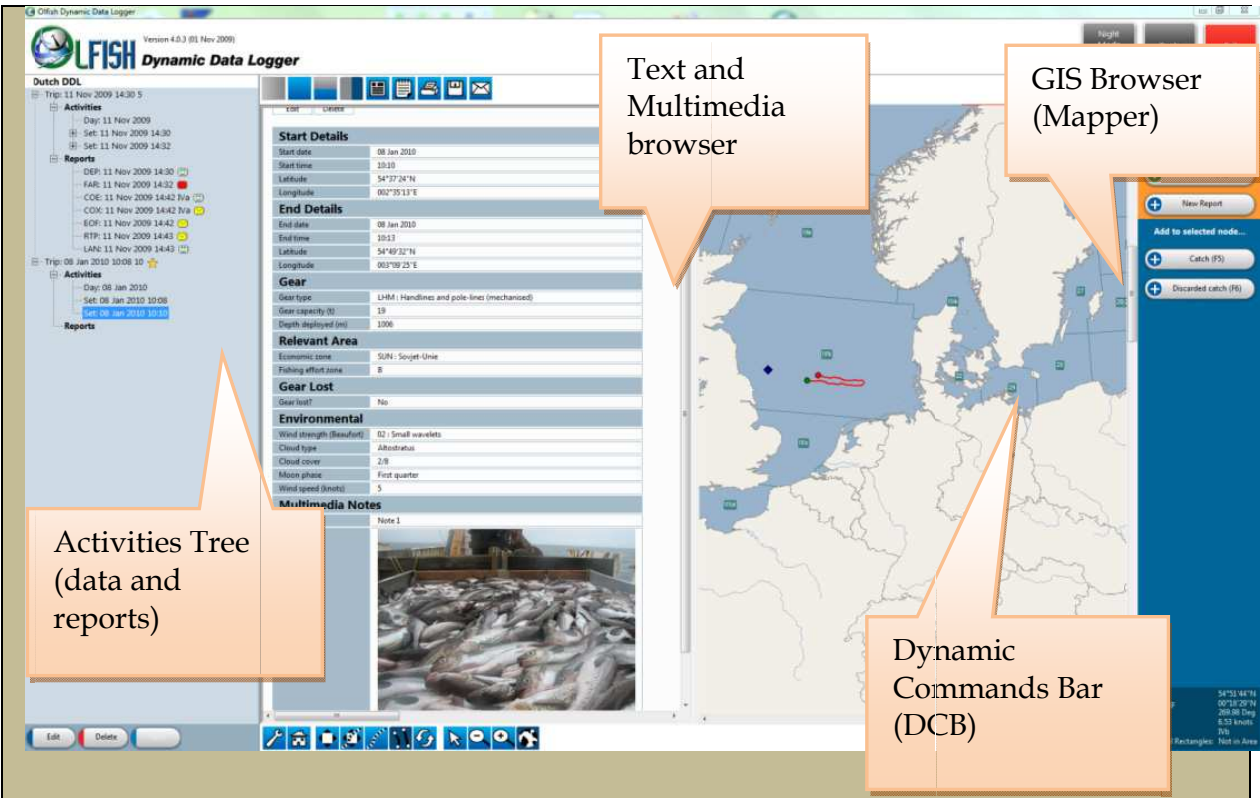
Fig. 5. Olfish-DDL main dashboard screen
