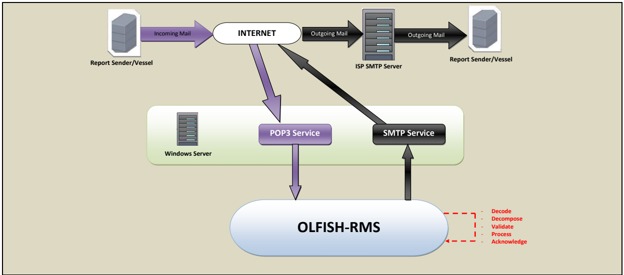
Fig. 29. Processor processes
