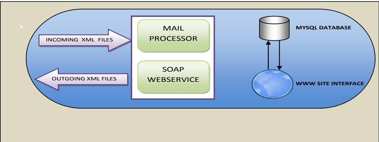
Fig. 28. Olfish-RMS components
