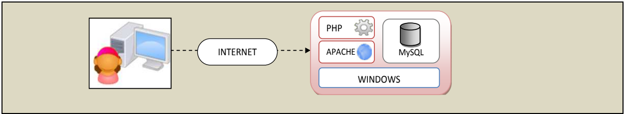
Fig. 27. Olfish-RMS infrastructure
