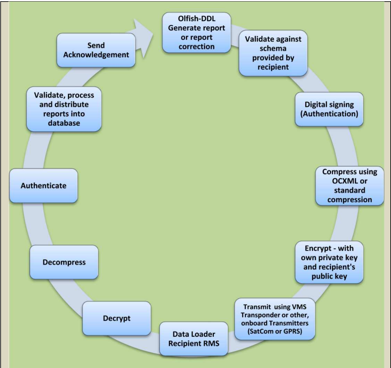
Fig. 12. Transmission process from Olfish-DDL to Shore-RMS
