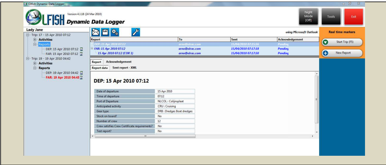
Fig. 11. Report Manager
