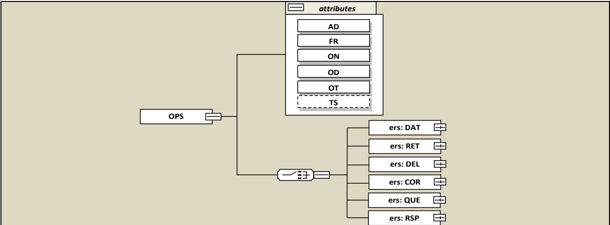
Fig. 30. Operations XSD
