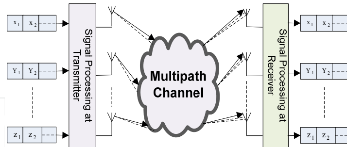
Fig. 1. The MIMO propagation channel.
