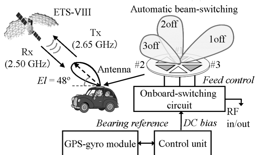
Fig. 5. Antenna system architecture
