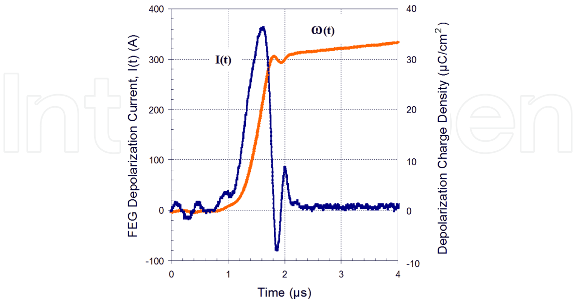
Fig. 9. Waveform of the pulsed depolarization current, I(t) , and the depolarization charge density, \omega(t) , released due to longitudinal shock compression of PZT 52/48 disk with D = 26.1 \text{ mm} / h = 0.65 \text{ mm} .
