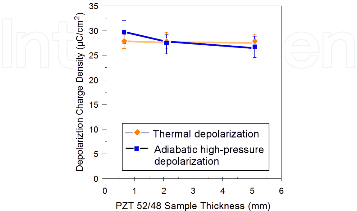
Fig. 11. Experimental data for the thermal and longitudinal explosive shock wave depolarization of PZT 52/48 samples.
