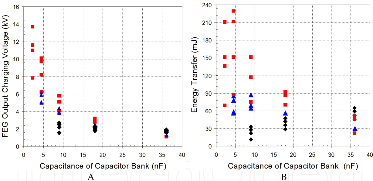
Fig. 15. Performance of FEG-Capacitor bank system. A - amplitude of the voltage pulse produced by FEGs across capacitor banks of different capacitance. B - energy delivered from FEGs to capacitor banks of different capacitance. PZT 52/48 elements of D = 26.1 mm/ h = 0.65 mm (diamonds), D = 27.0 mm/ h = 2.1 mm (triangles) and D = 25.4 mm/ h = 5.1 mm (squares).
