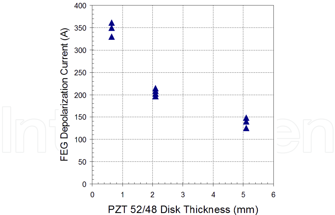
Fig. 10. Amplitude of shock induced depolarization current versus thickness of PZT 52/48 disks.
