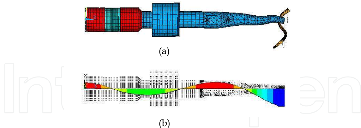
Fig. 4. (a) Deformed shape and (b) the axial vibration profile of the transducer at the 1.5\lambda axial mode (Lee, 2008; Lee et al., 2009).
