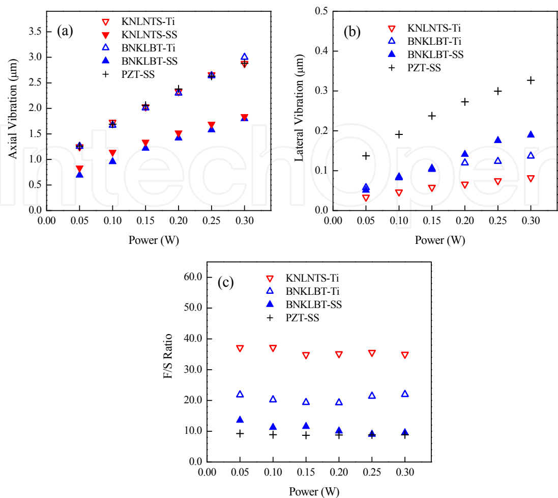
Fig. 10. Variations of (a) the vibration at the tip front, (b) the vibration at the tip side and (c) the F/S ration with input power. (Lee, 2008; Chan et al., 2008).
