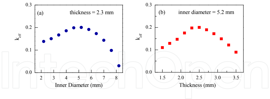
Fig. 3. Variations of k_{eff} with (a) inner diameter and (b) thickness for the KNLNTS ceramic ring (Lee, 2008).
