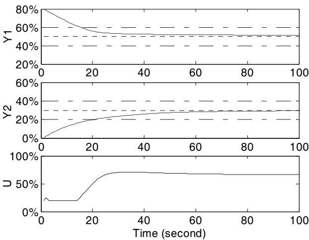
Fig. 15. NMPC based on PSMGA: priority order [A]
