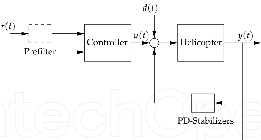
Fig. 17. Control setup for helicopter with inner stabilizing control loop and reference prefilter.
