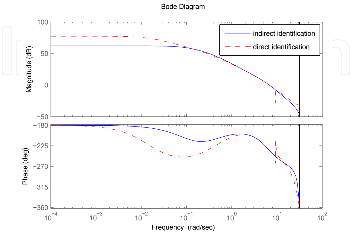
Fig. 8. Bode plot of models from direct and indirect approach
