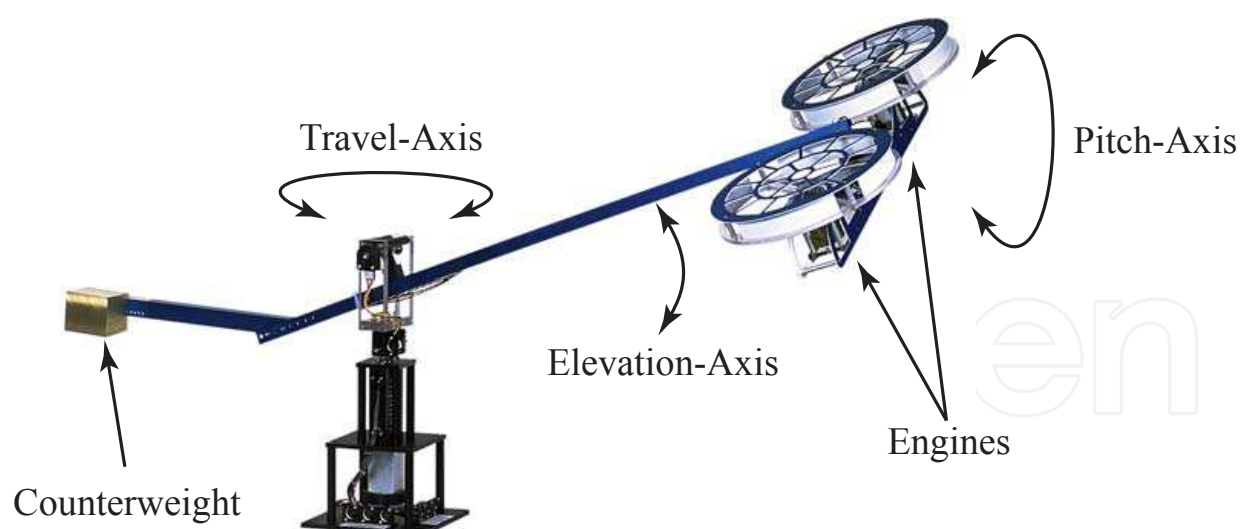
Fig. 1. Quanser 3-DOF Helicopter
