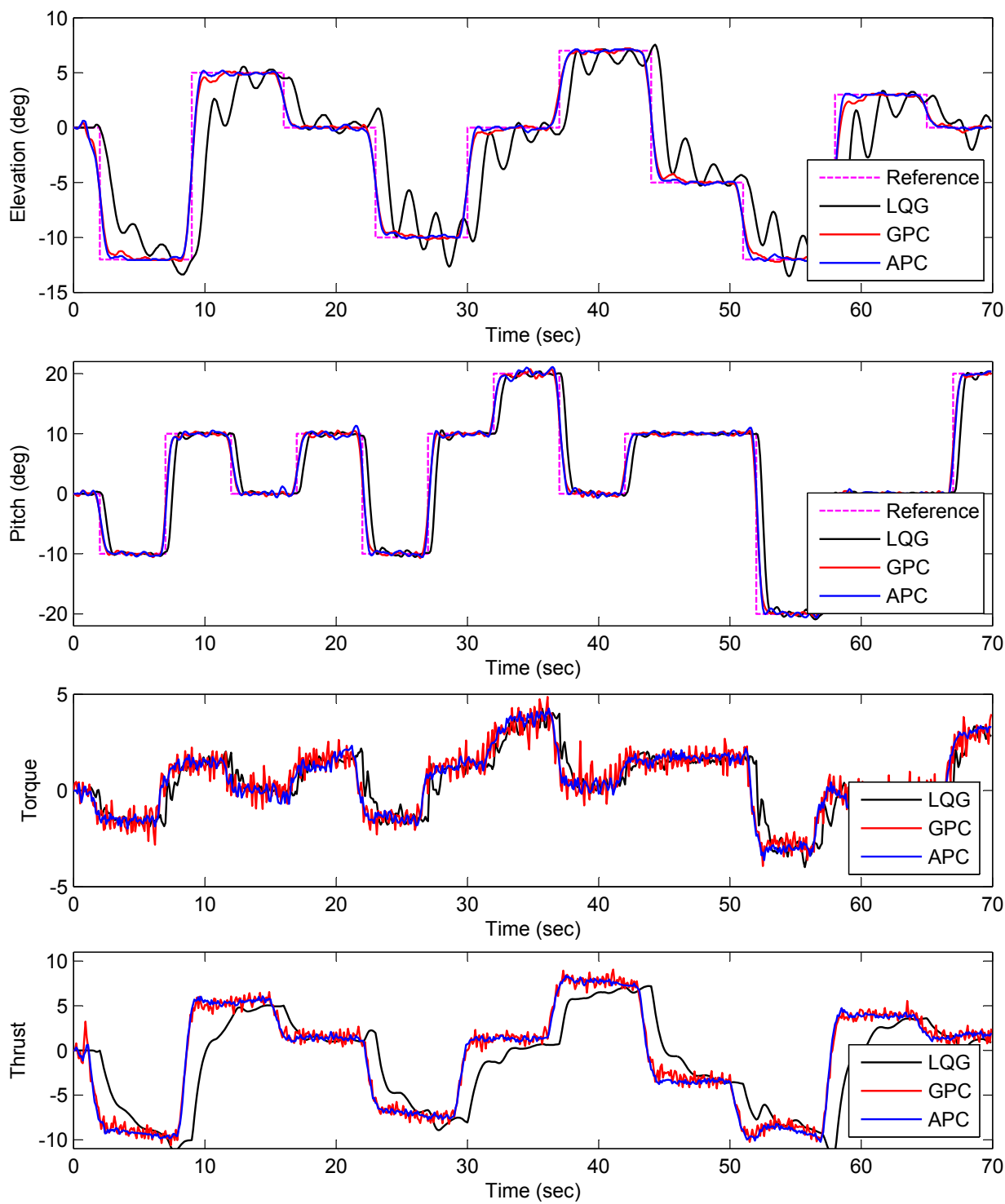
Fig. 18. Experimental results for tracking performance of APC compared to GPC and LQG. Top two plots: Control outputs. Bottom two plots: Control inputs.
