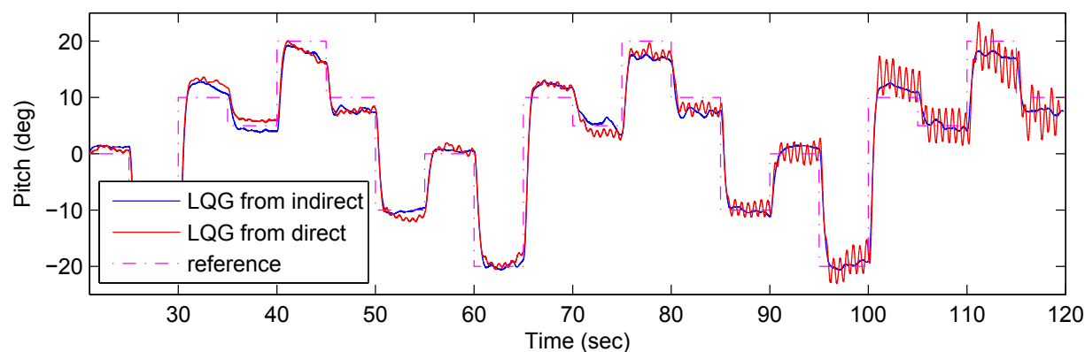
Fig. 10. Experimental results of controllers tracking a rectangular reference on the pitch axis. The LQG controller design was done with models from the direct and indirect approach respectively.
