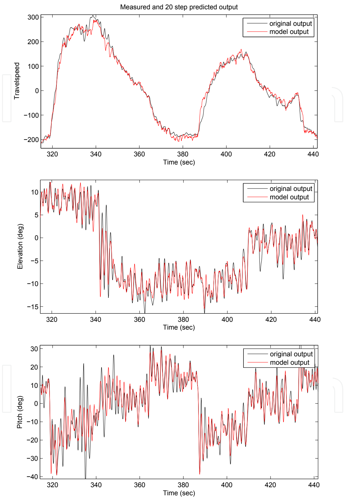
Fig. 11. 20-step ahead prediction output of the linear model for a validation data set
