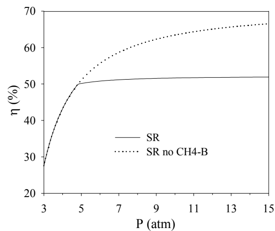
Fig. 9. \eta as a function of pressure for system with FP.C. Operating conditions: T_{SR}=600^{\circ}C , H_2O/CH_4=2.5 , SG/CH_4=0
