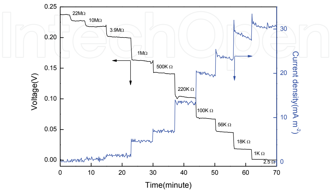
Fig. 4. Time courses of voltage associated with the current density readings of a PMFC with 4 cm electrode spacing after sequentially loading various resistances.
