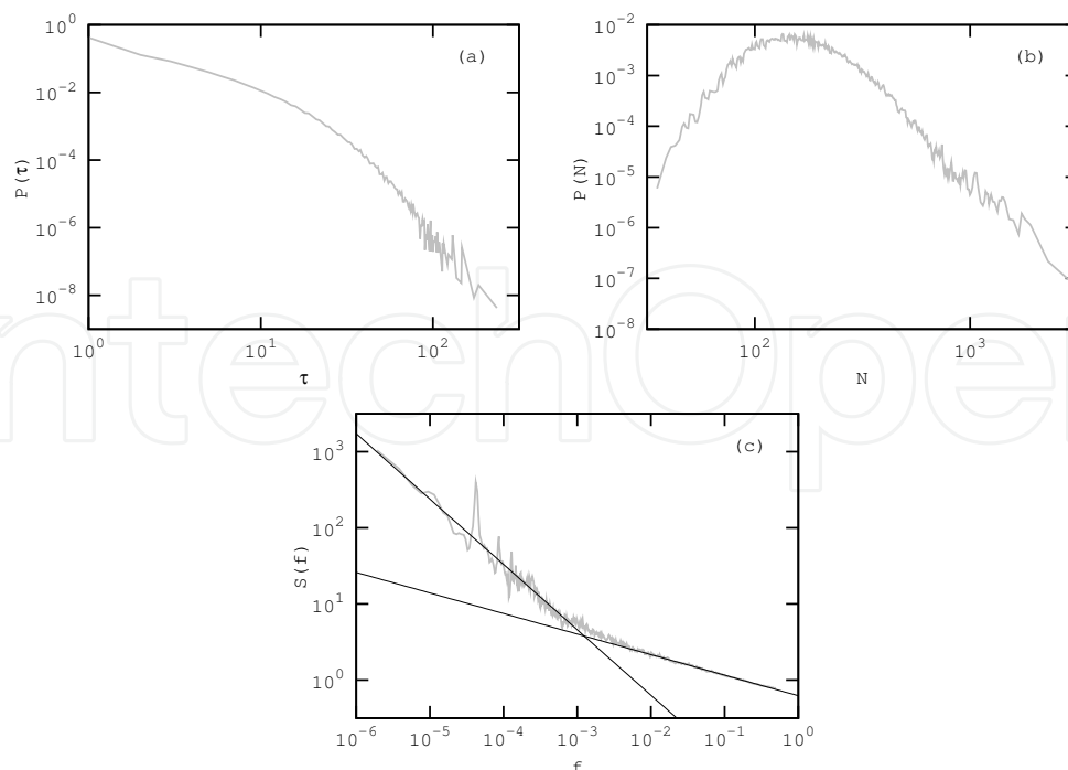
Fig. 2. Trading statistics of IBM stocks. (a) Empirical histogram of the inter-trade time \tau_k sequence, P(\tau) ; (b) histogram of trading activity, P(N) , calculated in the time interval \tau_d = 600 s; (c) PSD, S(f) , of the sequence of trades (gray curve), straight black lines approximate PSD S(f) \sim 1/f^{\beta_{1,2}} with \beta_1 = 0.33 and \beta_2 = 0.94 .
