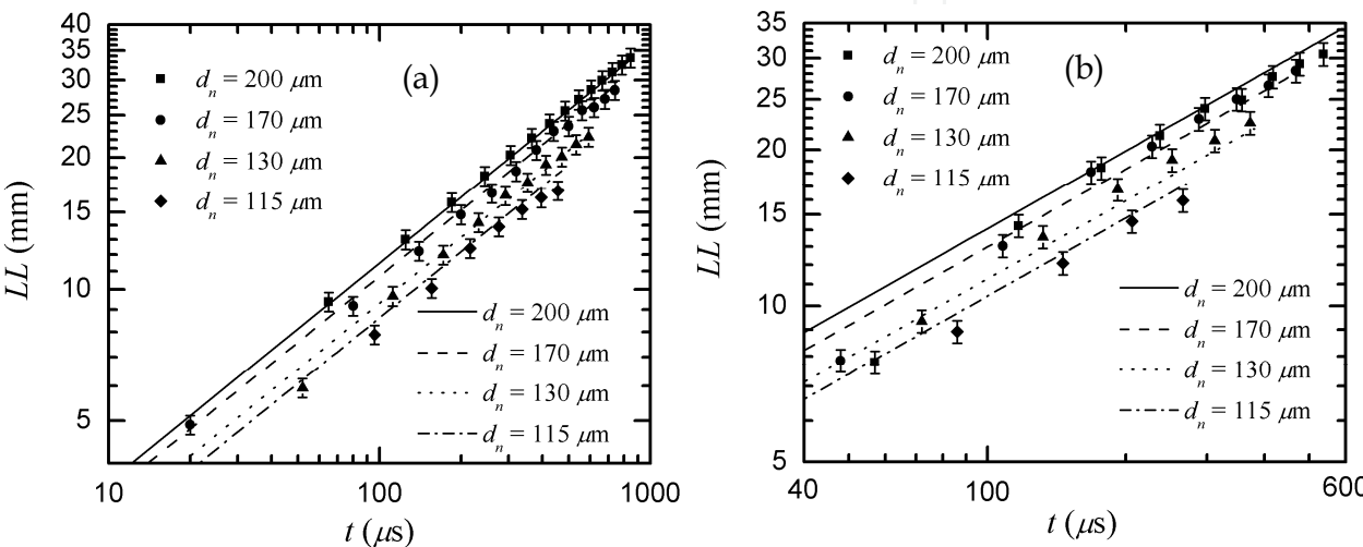
Fig. 9. Comparison between experimental data and the proposed correlation, equation 42. (a): P inj = 300 bar and (b): P inj = 700 bar, \rho_a = 26 \text{ kg/m}^3 and T_g = 906 \text{ K} .
