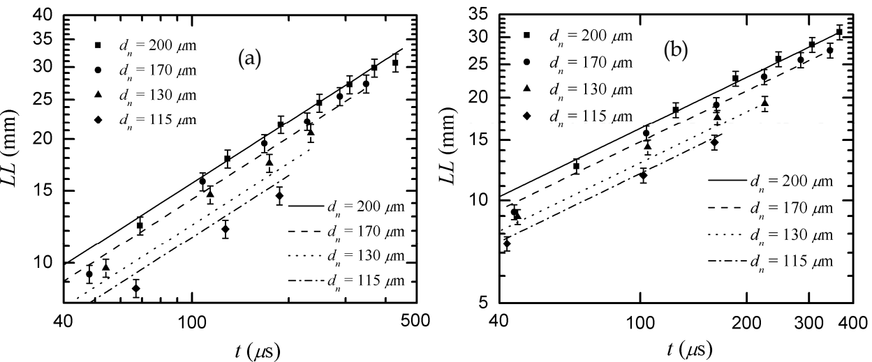
Fig. 10. Comparison between experimental data and the proposed correlation, equation 42. (a): P inj = 1100 bar and (b): P inj = 1300 bar, \rho_a = 26 \text{ kg/m}^3 and T_g = 906 \text{ K} .
