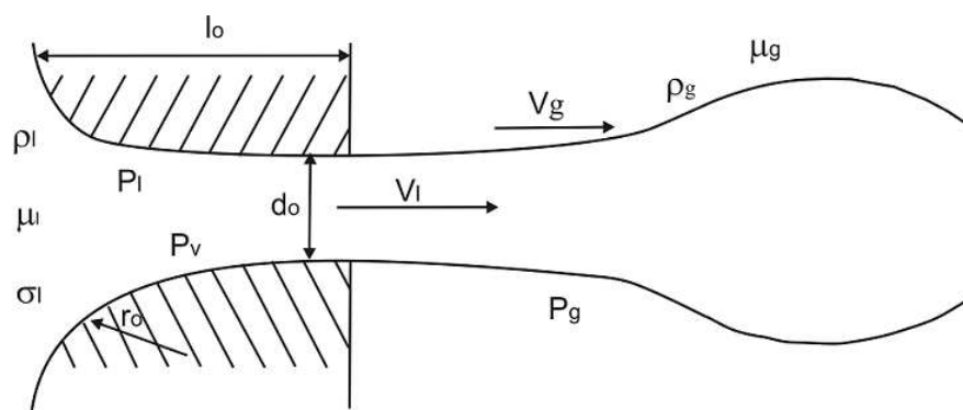
Fig. 1. Meaningful variables of the injection process.
