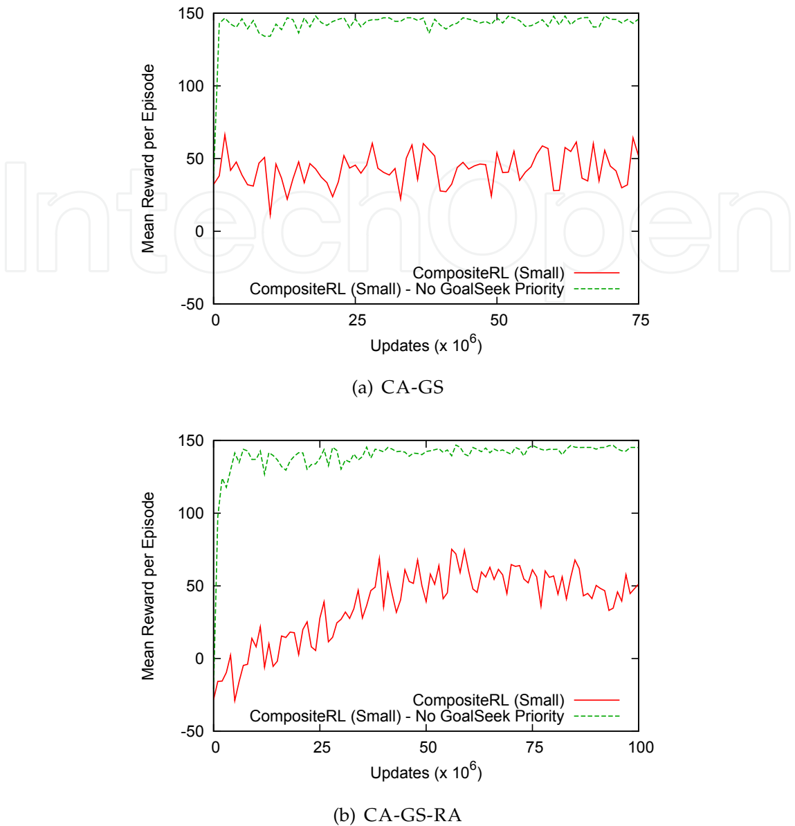
Fig. 14. Results on the validation set environments for the CA-GS and CA-GS-RA composite tasks comparing different approaches for the Small abstraction level.
