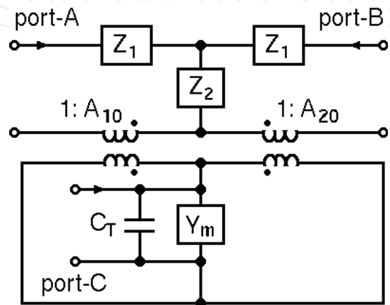
Fig. 3. Equivalent circuit model of IDT
