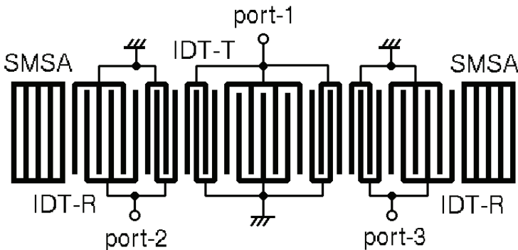
Fig. 7. Balanced SAW filter with pitch-modulated IDTs
