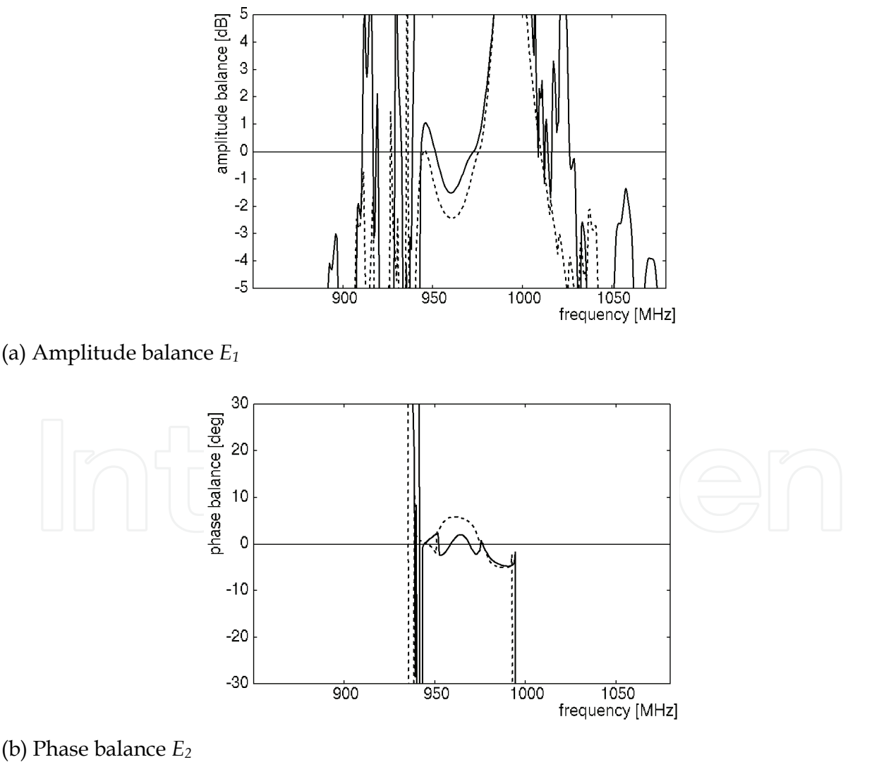
Fig. 10. Balance characteristics of the balanced SAW filter shown in Fig. 7
