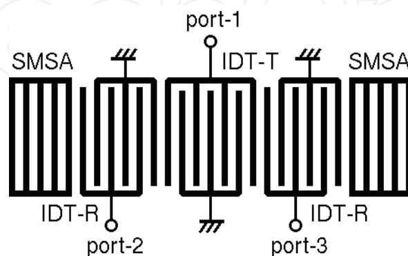
Fig. 1. Typical structure of the balanced SAW filter
