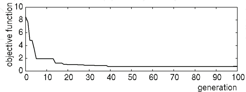
Fig. 9. Trajectory of the best objective function values ( D=15 ) By using the same values for the control parameters, the classic DE is applied to the extended optimum design problem of the balanced SAW filter. Table 3 compares the final best solution with the initial best solution in the same way with Table 2. Furthermore, Fig. 9 plots a representative example of the trajectory of the best objective function values in the
