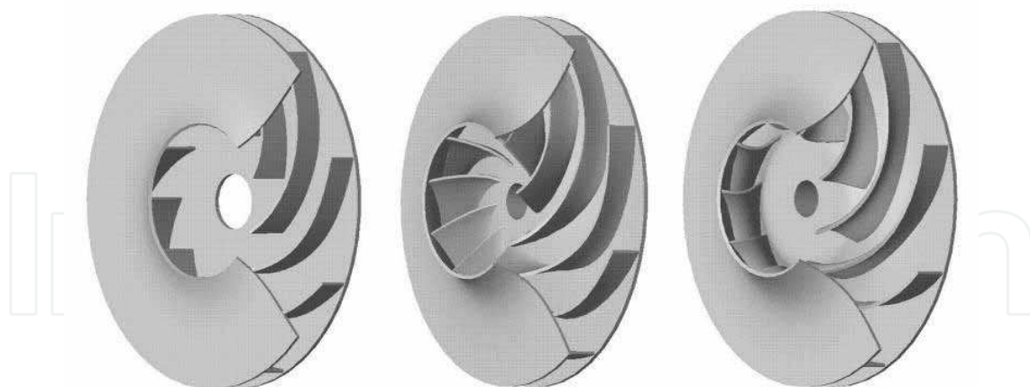
Fig. 11. The existent impeller (left), the worst optimized impeller (middle), and the best optimized impeller (right)
