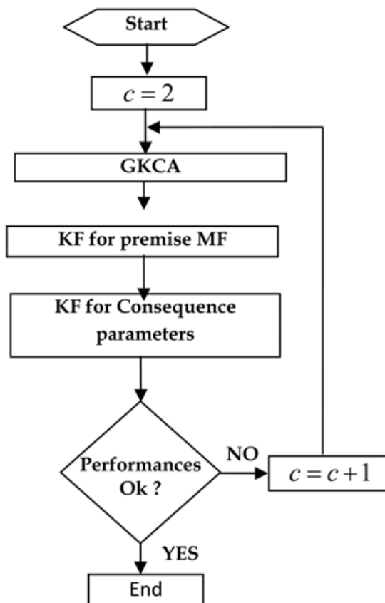
Fig. 6. Structure of the proposed fuzzy modeling
