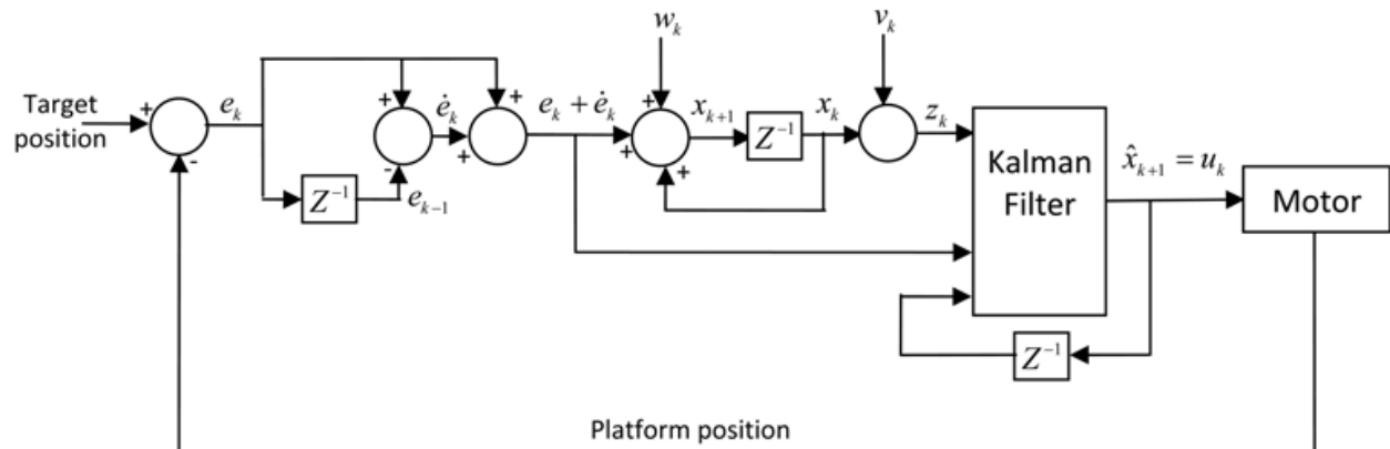
Fig. 3. Control system
