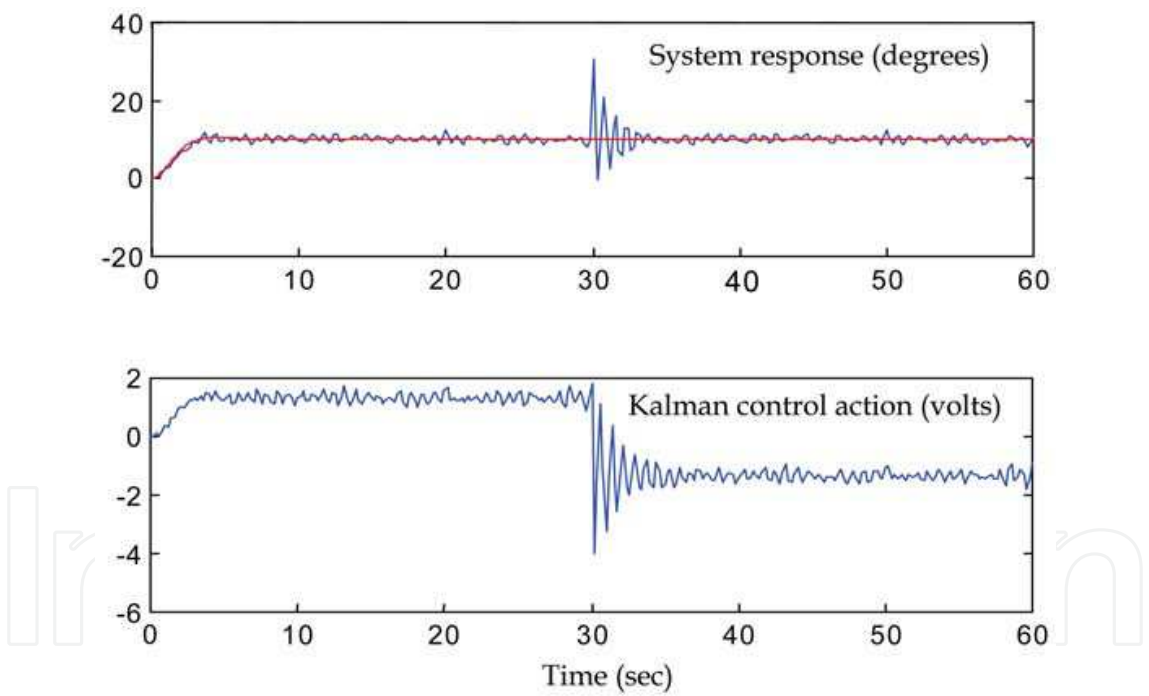
Fig. 5. System response and Kalman control action to a step input and a strong load disturbance
