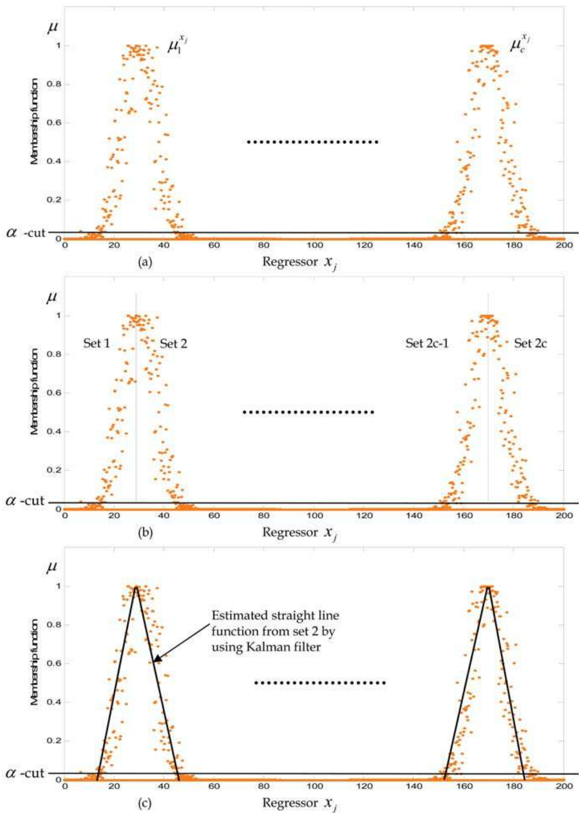
Fig. 7. Determination of premise membership functions : (a) Premiss MF defined point-wise for the regressors x_j, j=1,2,...n (b) Division of each membership function into 2 sets ( 2c sets are obtained for each x_j and 2cn sets are obtained for all regressors) (c) Approximation of each set by a straight line function by using Kalman filter
