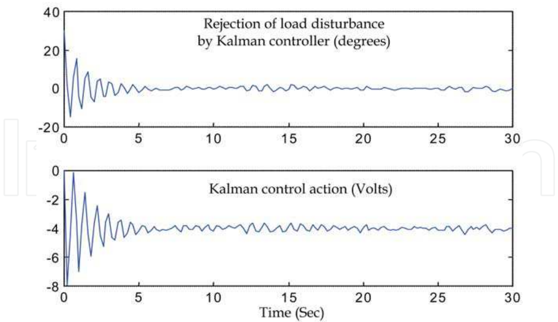
Fig. 4. System response and Kalman control action to a strong load disturbance
