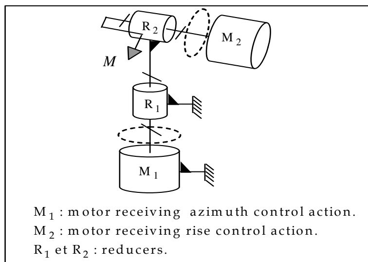
Fig. 1. Positioning system
