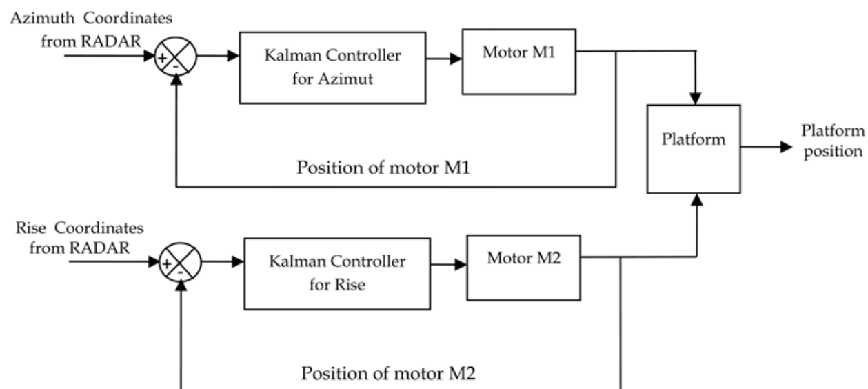
Fig. 2. Control system
