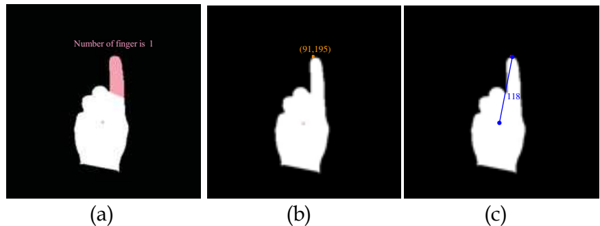
Fig. 16. An example of the feature extraction. (a) Number of fingers; (b) Fingertip's coordinate; (c) Finger-centroid distance.
