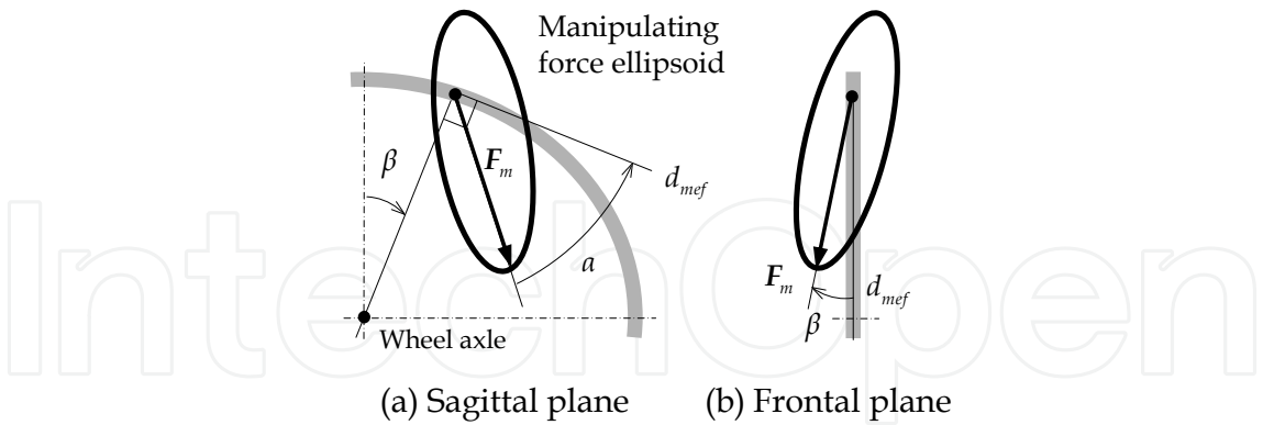
Fig. 13. Definition of component and angle of manipulating force ellipsoid.
