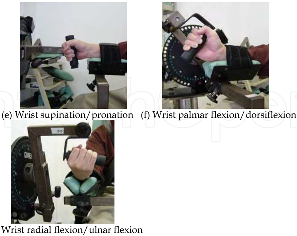
Fig. 4. Measurement of maximum joint torque.
