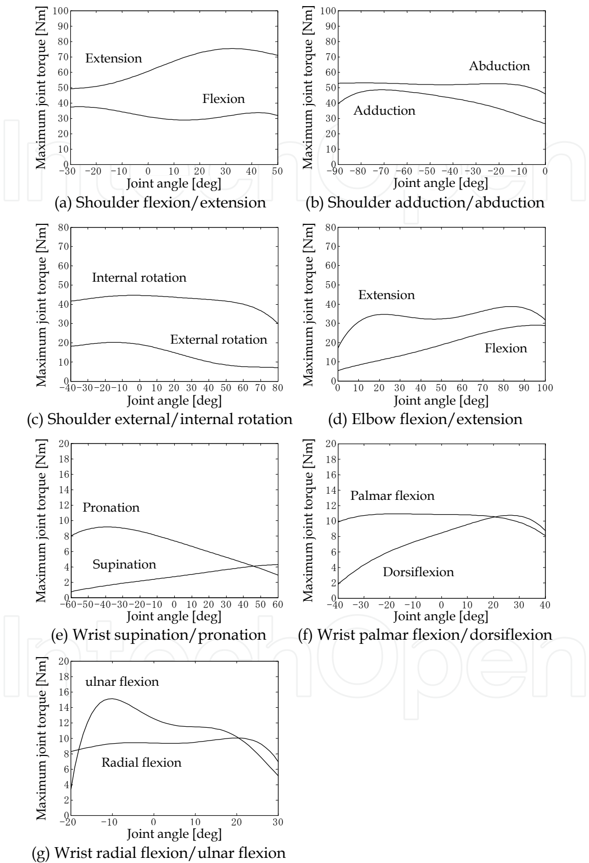
Fig. 6. Measurement results of maximum joint torque.
