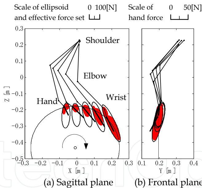
Fig. 17. Stick diagram of the upper limb, hand force, manipulating force ellipsoid, and driving force contribution figure.
