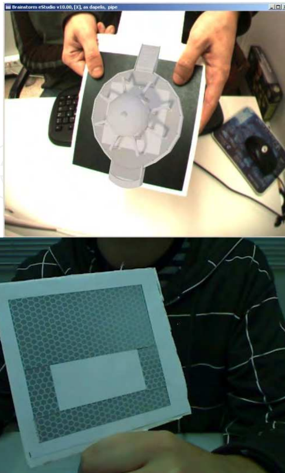
Fig. 3. (a) Left: Example of occlusion. (b) Right: ID-based markers with retro-reflective paper for supported infrared marker detection
