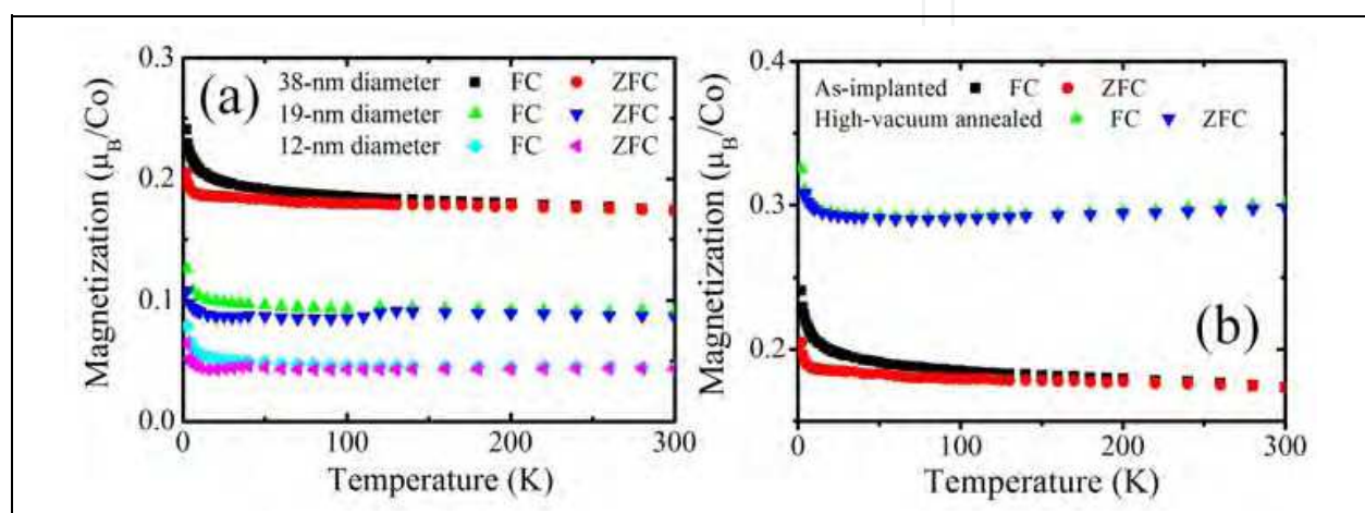
Fig. 9. (a) FC and ZFC behaviors of temperature dependent magnetization of as-implanted \text{Zn}_{0.92}\text{Co}_{0.08}\text{O} NWs with average diameters of 12, 19, and 38 nm. (b) FC and ZFC magnetizations of as-implanted and high-vacuum annealed \text{Zn}_{0.92}\text{Co}_{0.08}\text{O} NWs with an average diameter of 38 nm. The annealing time is 12 h.
