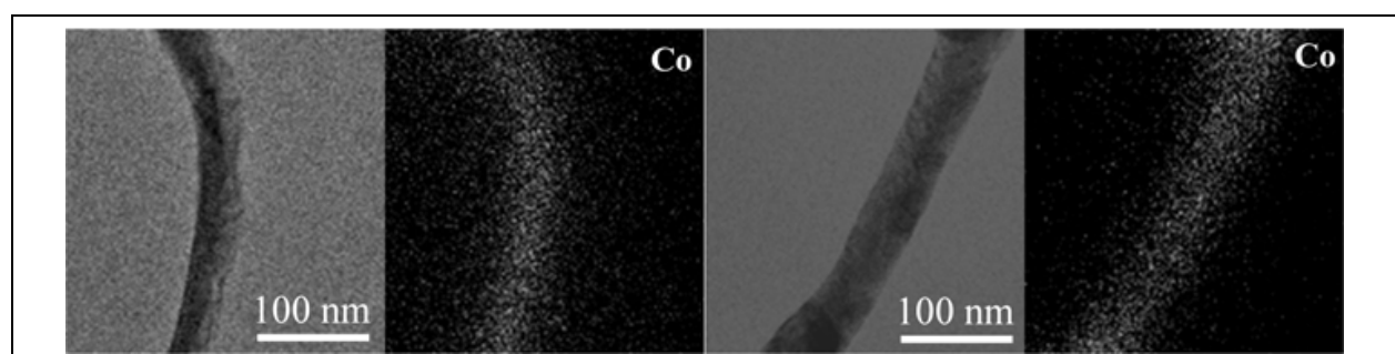
Fig. 7. TEM images of (a) as-implanted and (c) high-vacuum annealed \text{Zn}_{1-x}\text{Co}_x\text{O} NWs with a dose of 6 \times 10^{16} \text{ cm}^{-2} and an average diameter of 38 nm. EDX mapping images of the Co element in (b) as-implanted and (d) high-vacuum annealed \text{Zn}_{1-x}\text{Co}_x\text{O} NWs.
