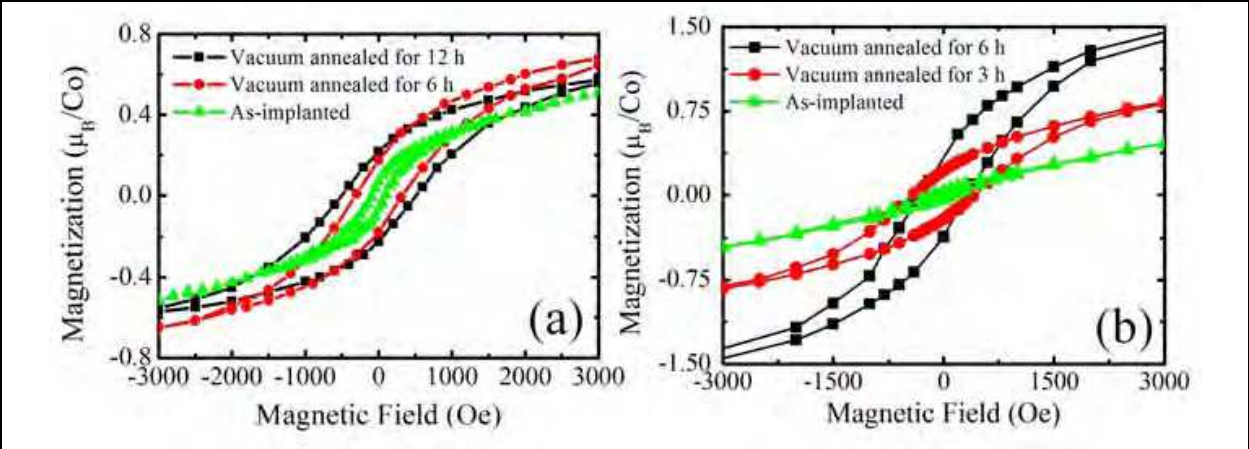
Fig. 12. (a) Hysteresis loops, taken at 10 K, of as-implanted, 6-h vacuum annealed, and 12-h vacuum annealed Zn 0.92 Co 0.08 O NWs with a 38-nm average diameter. (b) Hysteresis loops, taken at 2 K, of as-implanted, 3-h vacuum annealed, and 6-h vacuum annealed Zn 0.92 Co 0.08 O NWs with a 19-nm average diameter.
