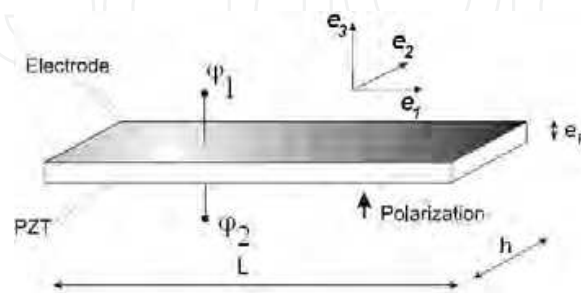
Fig. 5. Thickness-polarized piezoelectric beam transducer with electroded surfaces, and orientation in the material reference frame ( e_1, e_2, e_3 ). \phi_1 and \phi_2 denotes the electric potential of the electrodes.
