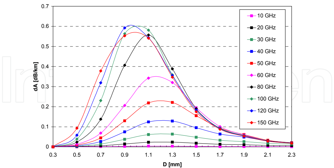
Fig. 10. Contribution of rain drops of diameter D to the specific rain attenuation; transmission frequency is a parameter
