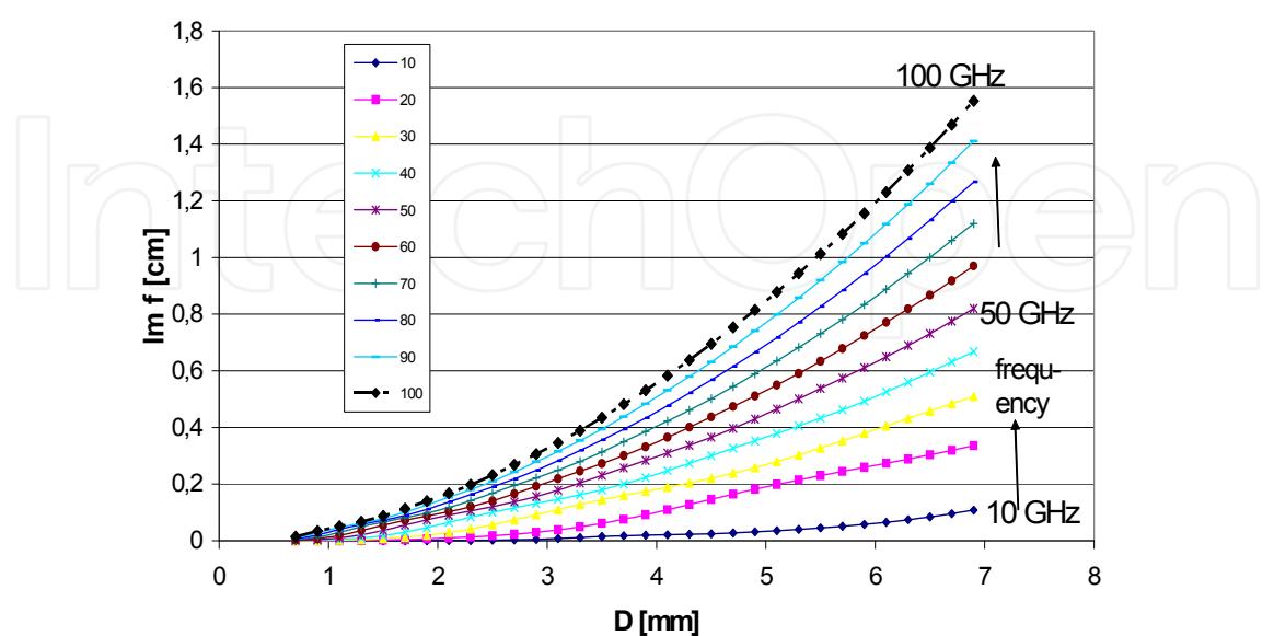
Fig. 8. Imaginary parts of forward scattering functions being proportional to the rain attenuation
