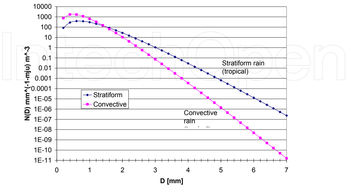
Fig. 2. Gamma DSD model using parameters from Table 1 for certain rain rate value
