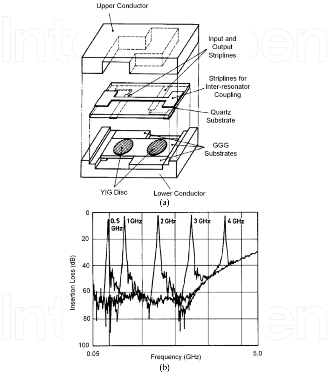
Fig. 11. Tunable bandpass filter using ferromagnetic disks a) filter structure b) filter response, taken from (Murakami et al., 1987)
