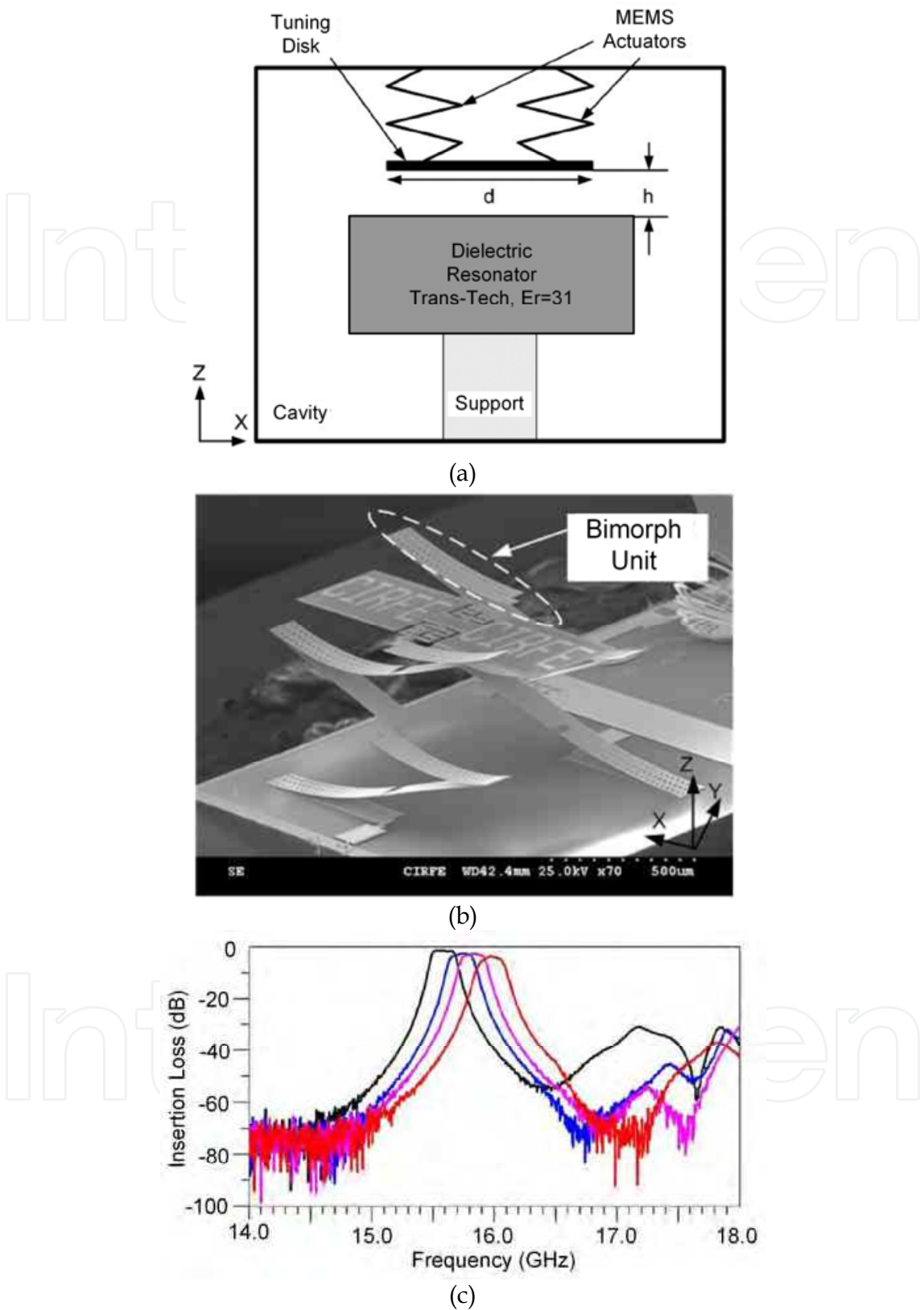
Fig. 12. Tunable bandpass filter using dielectric resonators and MEMS thermal actuators a) tuning structure schematic b) MEMS thermal actuator isotropic view c) filter response, taken from (Yan & Mansour, 2007 a)
