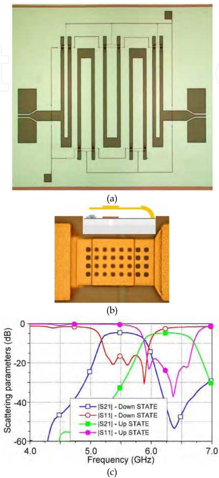
Fig. 7. Tunable bandpass filter using direct contact MEMS cantilever switches a) photography b) direct contact MEMS cantilever switch c) filter response, taken from (Ocera et al., 2006)
