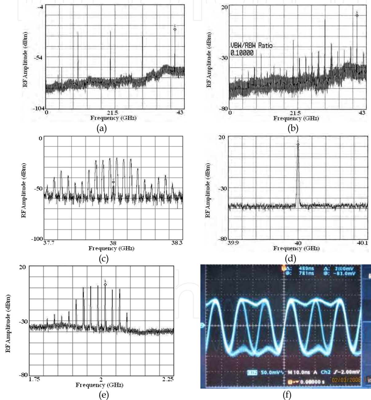
Fig. 10. The electrical spectrum of (a) generated harmonics at D, (b) at D when 2-GHz IF signal is added, (c) 38-GHz BPSK at E, (d) 40-GHz signal at J, (e) 2-GHz BPSK at O, (f) Waveform of demodulated 100-Mbps Ethernet data.
