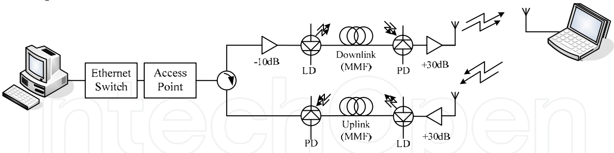
Fig. 3. The experimental setup of direct intensity modulation.
