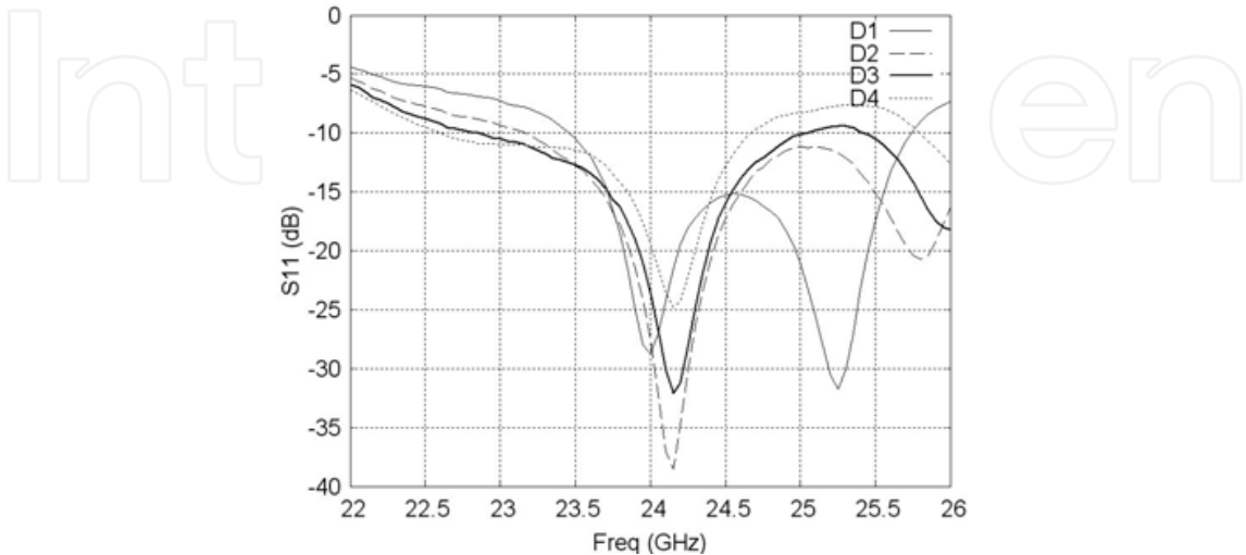
Fig. 12. Passive HPBW antenna – Measured S11 results for all configurations
